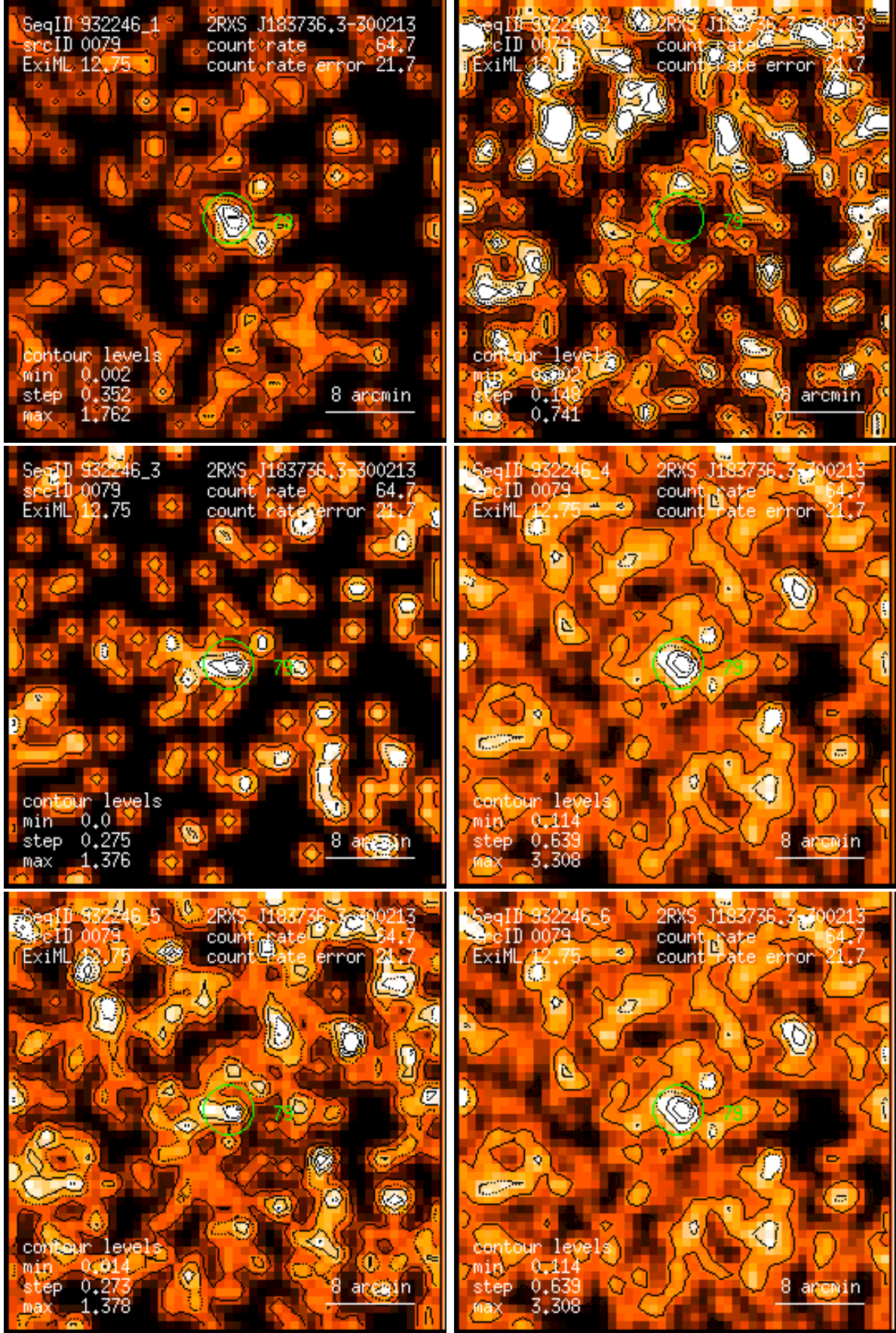
Figure 79: RASS 932246: detection 0079: band rate images, Gaussian filter: (1) PSPC channels 11 – 41, (2) 52 – 90, (3) 91 – 201, (4) 11 – 235, (5) 52 – 201, (6) 11 – 201. Broad band rates in counts/ks. Band rate contour levels in counts/ks/arcmin 2 .
