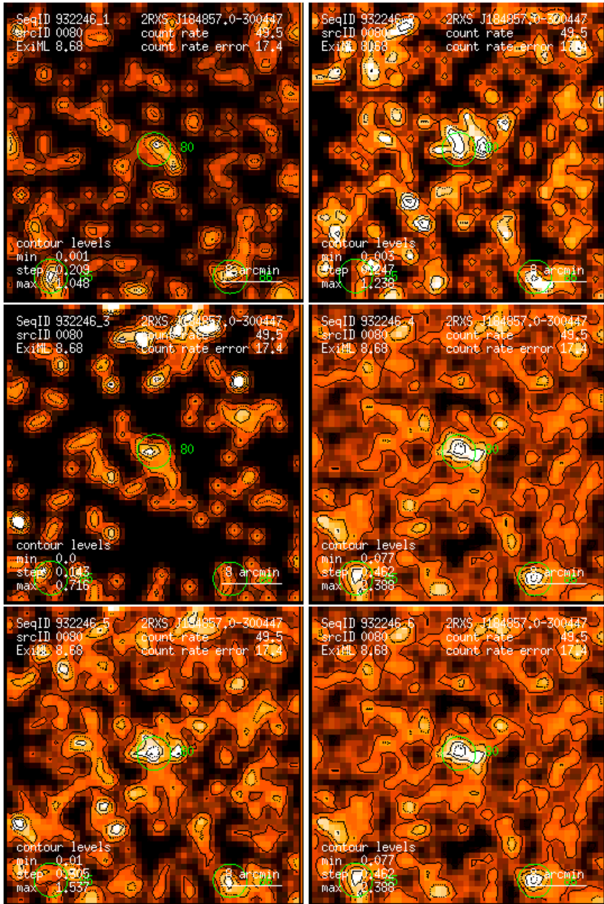
Figure 80: RASS 932246: detection 0080: band rate images, Gaussian filter: (1) PSPC channels 11 – 41, (2) 52 – 90, (3) 91 – 201, (4) 11 – 235, (5) 52 – 201, (6) 11 – 201. Broad band rates in counts/ks. Band rate contour levels in counts/ks/arcmin 2 .
