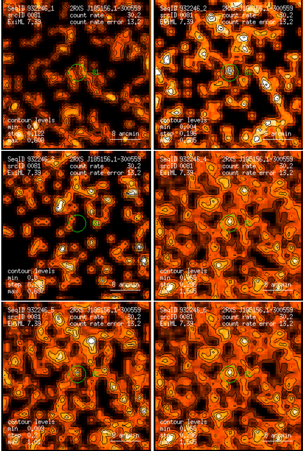
Figure 81: RASS 932246: detection 0081: band rate images, Gaussian filter: (1) PSPC channels 11 – 41, (2) 52 – 90, (3) 91 – 201, (4) 11 – 235, (5) 52 – 201, (6) 11 – 201. Broad band rates in counts/ks. Band rate contour levels in counts/ks/arcmin 2 .
