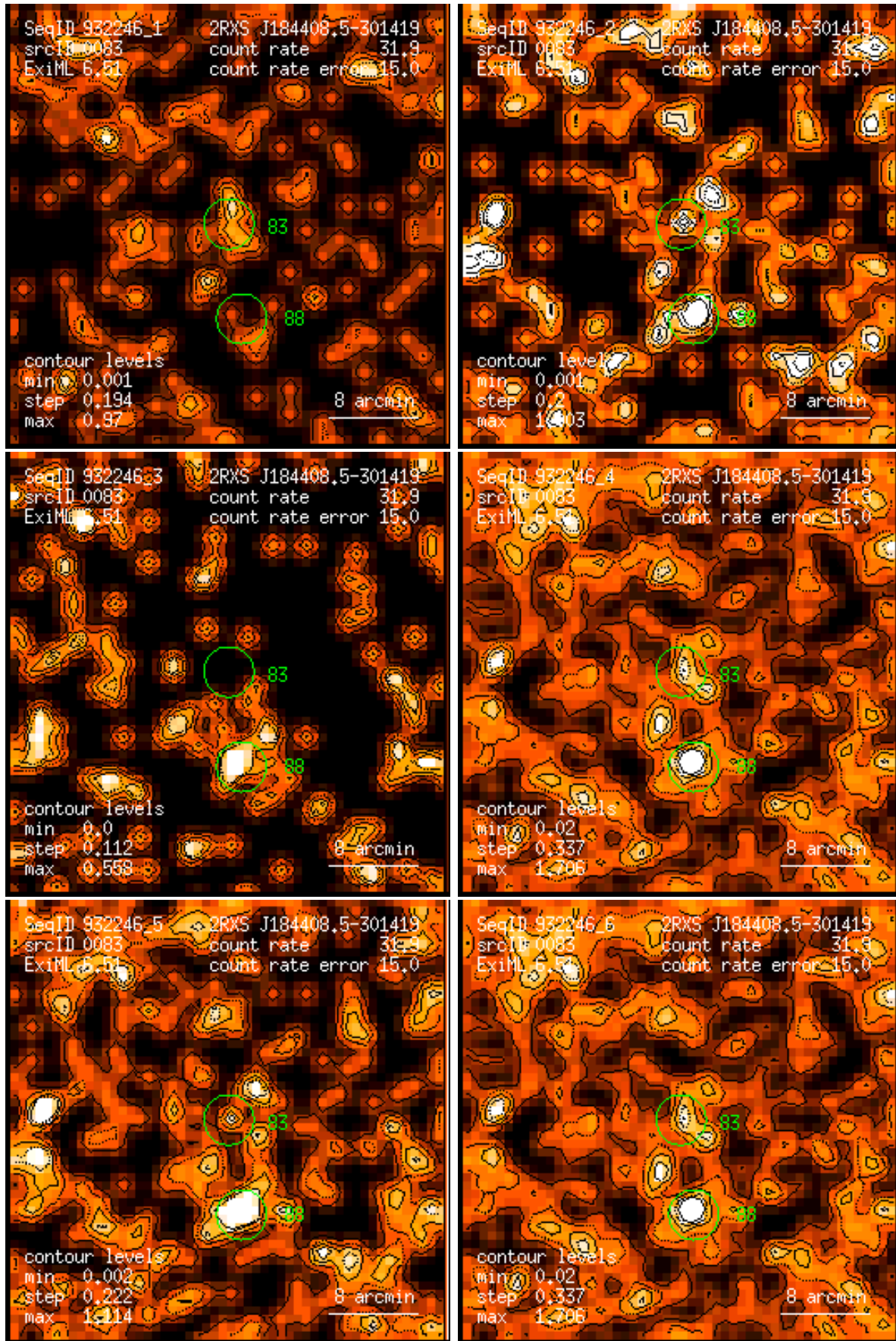
Figure 83: RASS 932246: detection 0083: band rate images, Gaussian filter: (1) PSPC channels 11 – 41, (2) 52 – 90, (3) 91 – 201, (4) 11 – 235, (5) 52 – 201, (6) 11 – 201. Broad band rates in counts/ks. Band rate contour levels in counts/ks/arcmin 2 .
