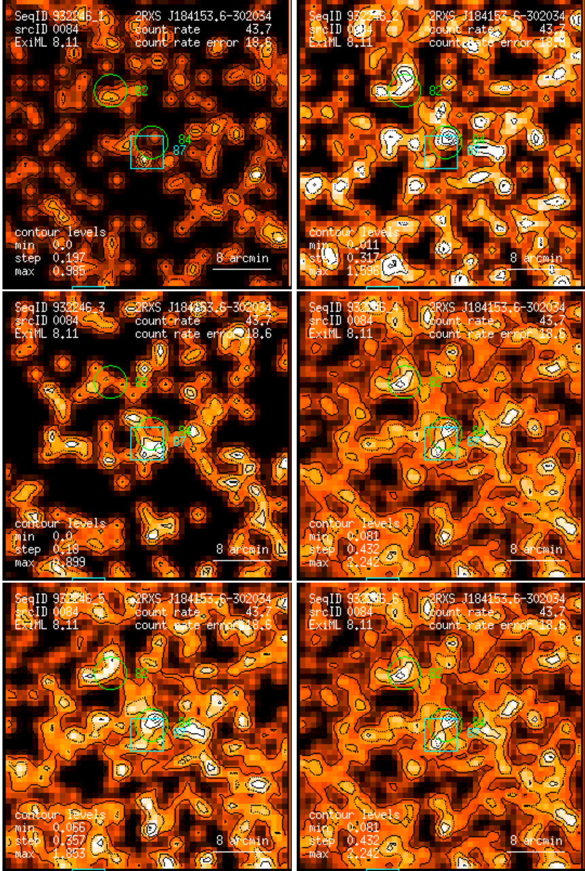
Figure 84: RASS 932246: detection 0084: band rate images, Gaussian filter: (1) PSPC channels 11 – 41, (2) 52 – 90, (3) 91 – 201, (4) 11 – 235, (5) 52 – 201, (6) 11 – 201. Broad band rates in counts/ks. Band rate contour levels in counts/ks/arcmin 2 .
