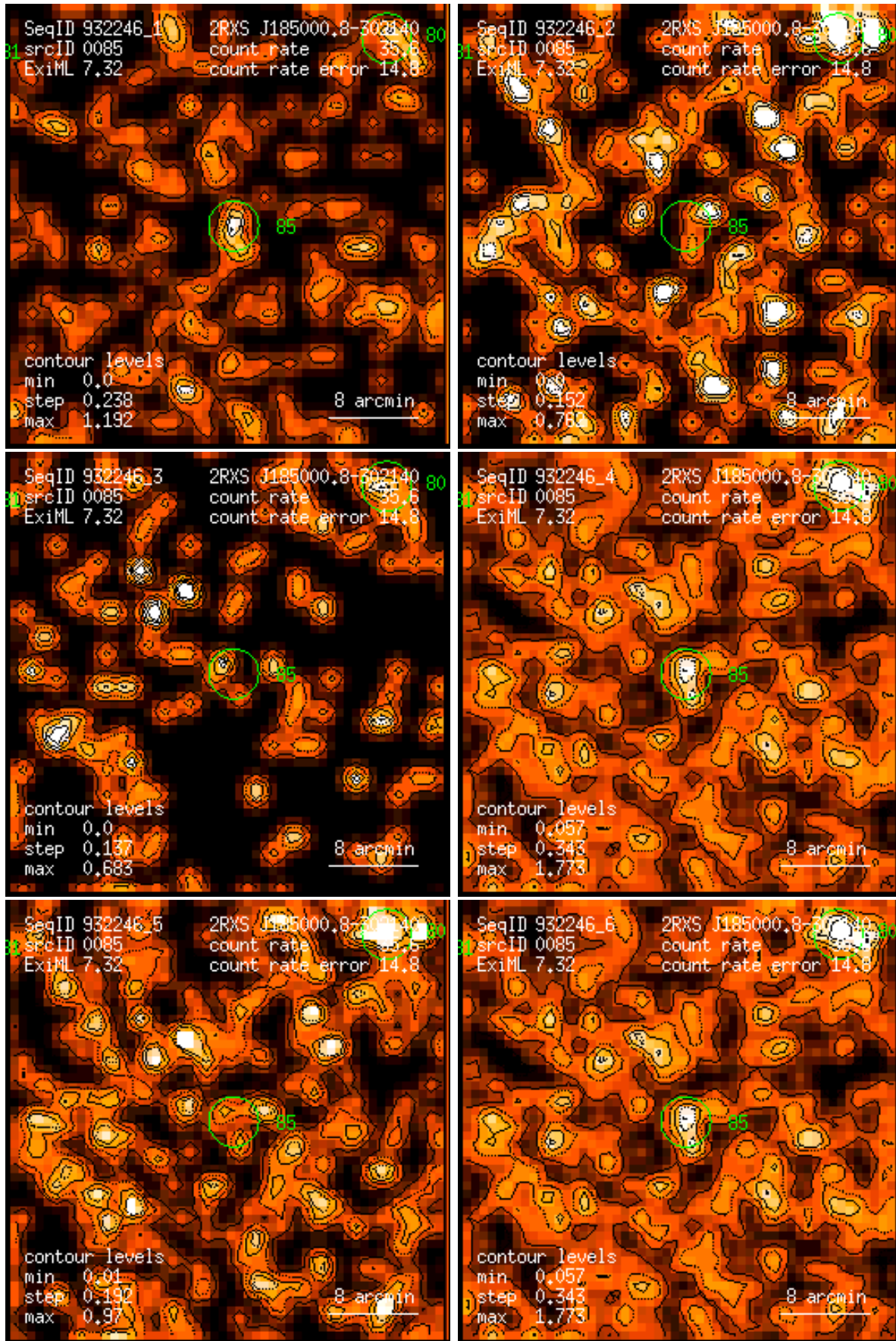
Figure 85: RASS 932246: detection 0085: band rate images, Gaussian filter: (1) PSPC channels 11 – 41, (2) 52 – 90, (3) 91 – 201, (4) 11 – 235, (5) 52 – 201, (6) 11 – 201. Broad band rates in counts/ks. Band rate contour levels in counts/ks/arcmin 2 .
