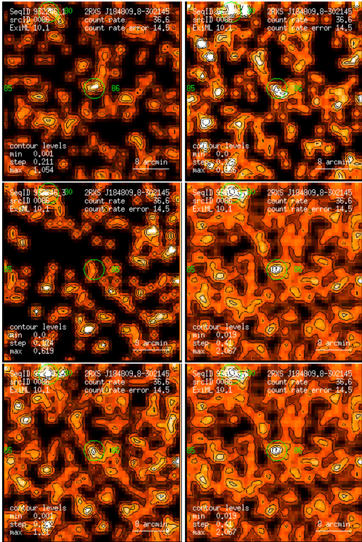
Figure 86: RASS 932246: detection 0086: band rate images, Gaussian filter: (1) PSPC channels 11 – 41, (2) 52 – 90, (3) 91 – 201, (4) 11 – 235, (5) 52 – 201, (6) 11 – 201. Broad band rates in counts/ks. Band rate contour levels in counts/ks/arcmin 2 .
