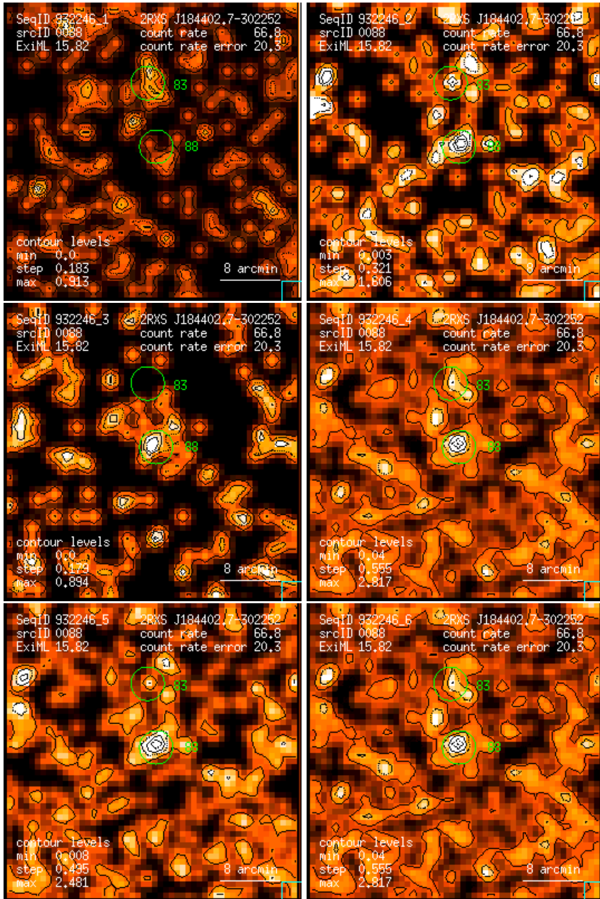
Figure 88: RASS 932246: detection 0088: band rate images, Gaussian filter: (1) PSPC channels 11 – 41, (2) 52 – 90, (3) 91 – 201, (4) 11 – 235, (5) 52 – 201, (6) 11 – 201. Broad band rates in counts/ks. Band rate contour levels in counts/ks/arcmin 2 .
