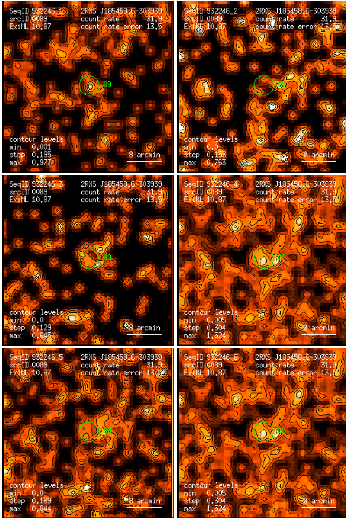
Figure 89: RASS 932246: detection 0089: band rate images, Gaussian filter: (1) PSPC channels 11 – 41, (2) 52 – 90, (3) 91 – 201, (4) 11 – 235, (5) 52 – 201, (6) 11 – 201. Broad band rates in counts/ks. Band rate contour levels in counts/ks/arcmin 2 .
