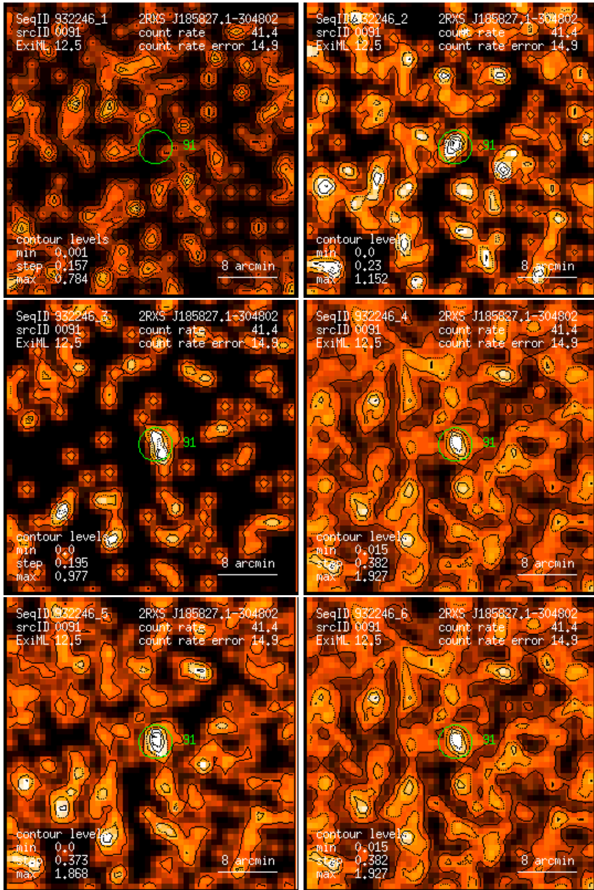
Figure 91: RASS 932246: detection 0091: band rate images, Gaussian filter: (1) PSPC channels 11 – 41, (2) 52 – 90, (3) 91 – 201, (4) 11 – 235, (5) 52 – 201, (6) 11 – 201. Broad band rates in counts/ks. Band rate contour levels in counts/ks/arcmin 2 .
