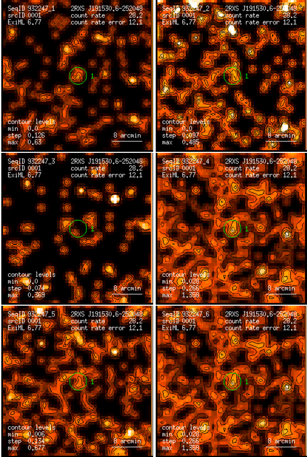
Figure 1: RASS 932247: detection 0001: band rate images, Gaussian filter: (1) PSPC channels 11 – 41, (2) 52 – 90, (3) 91 – 201, (4) 11 – 235, (5) 52 – 201, (6) 11 – 201. Broad band rates in counts/ks. Band rate contour levels in counts/ks/arcmin 2 .
