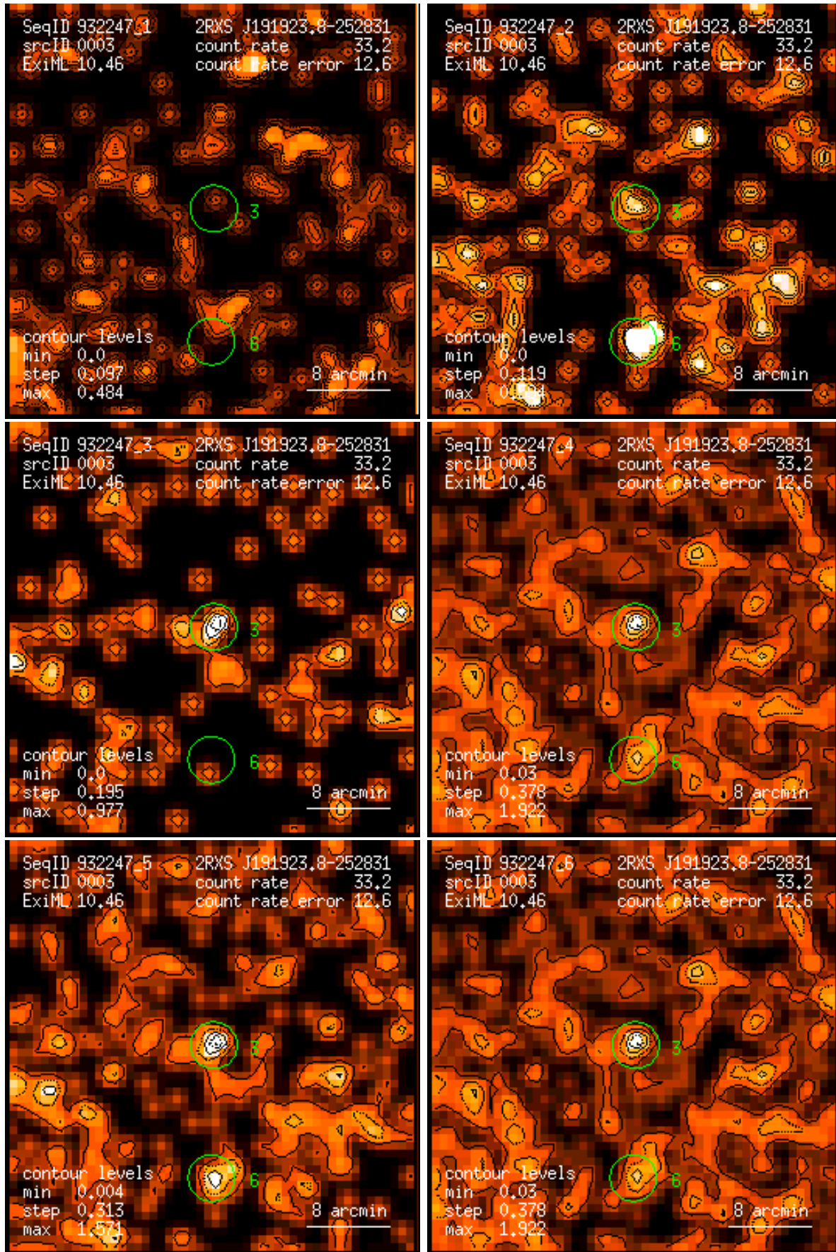
Figure 3: RASS 932247: detection 0003: band rate images, Gaussian filter: (1) PSPC channels 11 – 41, (2) 52 – 90, (3) 91 – 201, (4) 11 – 235, (5) 52 – 201, (6) 11 – 201. Broad band rates in counts/ks. Band rate contour levels in counts/ks/arcmin 2 .
