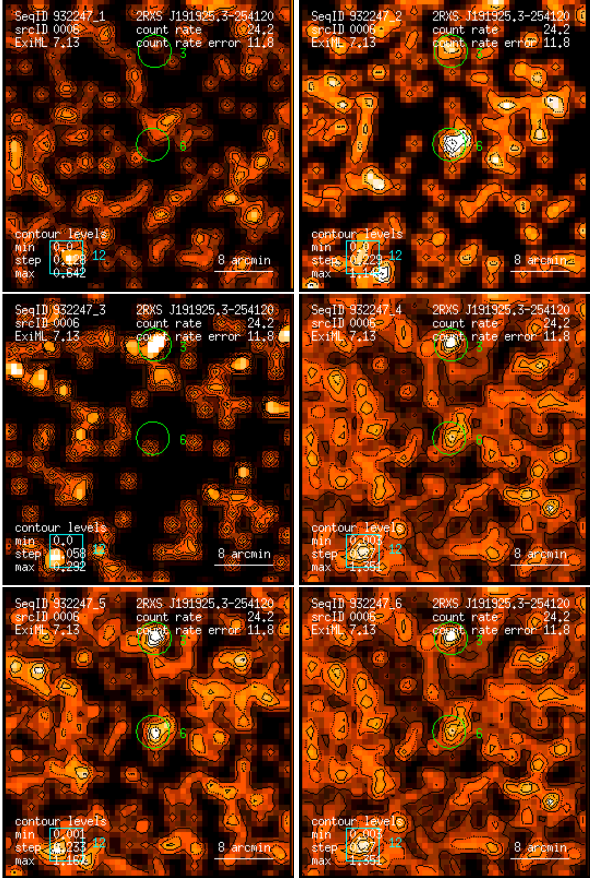
Figure 6: RASS 932247: detection 0006: band rate images, Gaussian filter: (1) PSPC channels 11 – 41, (2) 52 – 90, (3) 91 – 201, (4) 11 – 235, (5) 52 – 201, (6) 11 – 201. Broad band rates in counts/ks. Band rate contour levels in counts/ks/arcmin 2 .
