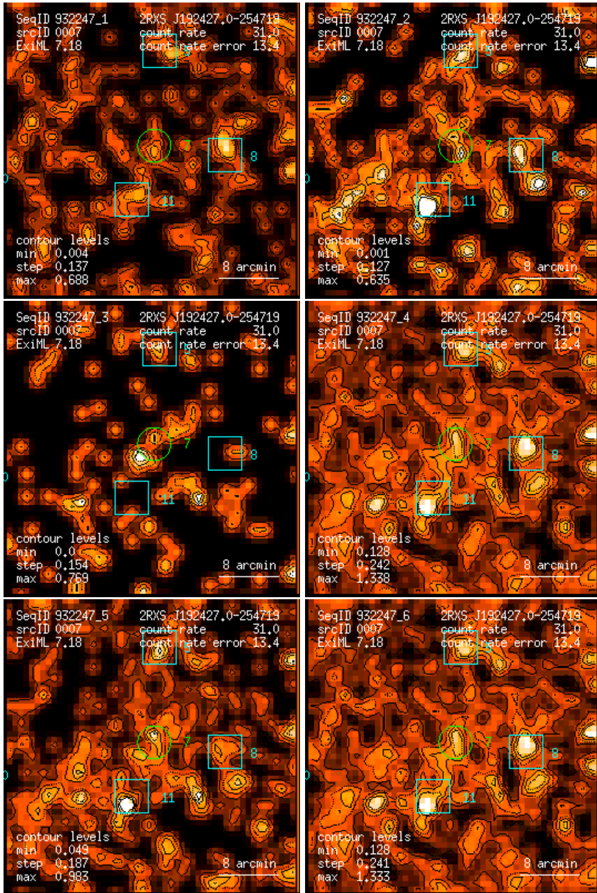
Figure 7: RASS 932247: detection 0007: band rate images, Gaussian filter: (1) PSPC channels 11 – 41, (2) 52 – 90, (3) 91 – 201, (4) 11 – 235, (5) 52 – 201, (6) 11 – 201. Broad band rates in counts/ks. Band rate contour levels in counts/ks/arcmin 2 .
