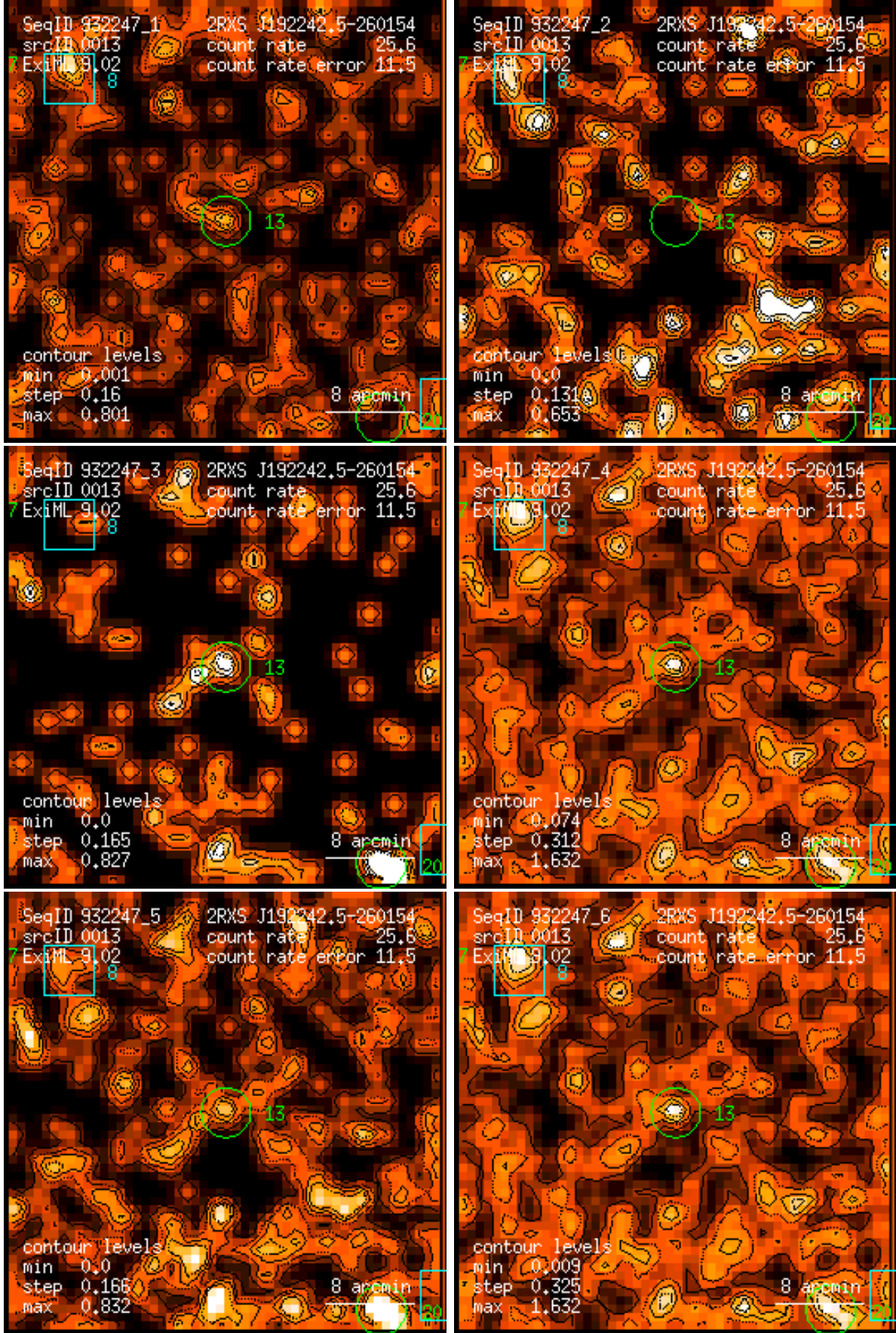
Figure 13: RASS 932247: detection 0013: band rate images, Gaussian filter: (1) PSPC channels 11 – 41, (2) 52 – 90, (3) 91 – 201, (4) 11 – 235, (5) 52 – 201, (6) 11 – 201. Broad band rates in counts/ks. Band rate contour levels in counts/ks/arcmin 2 .
