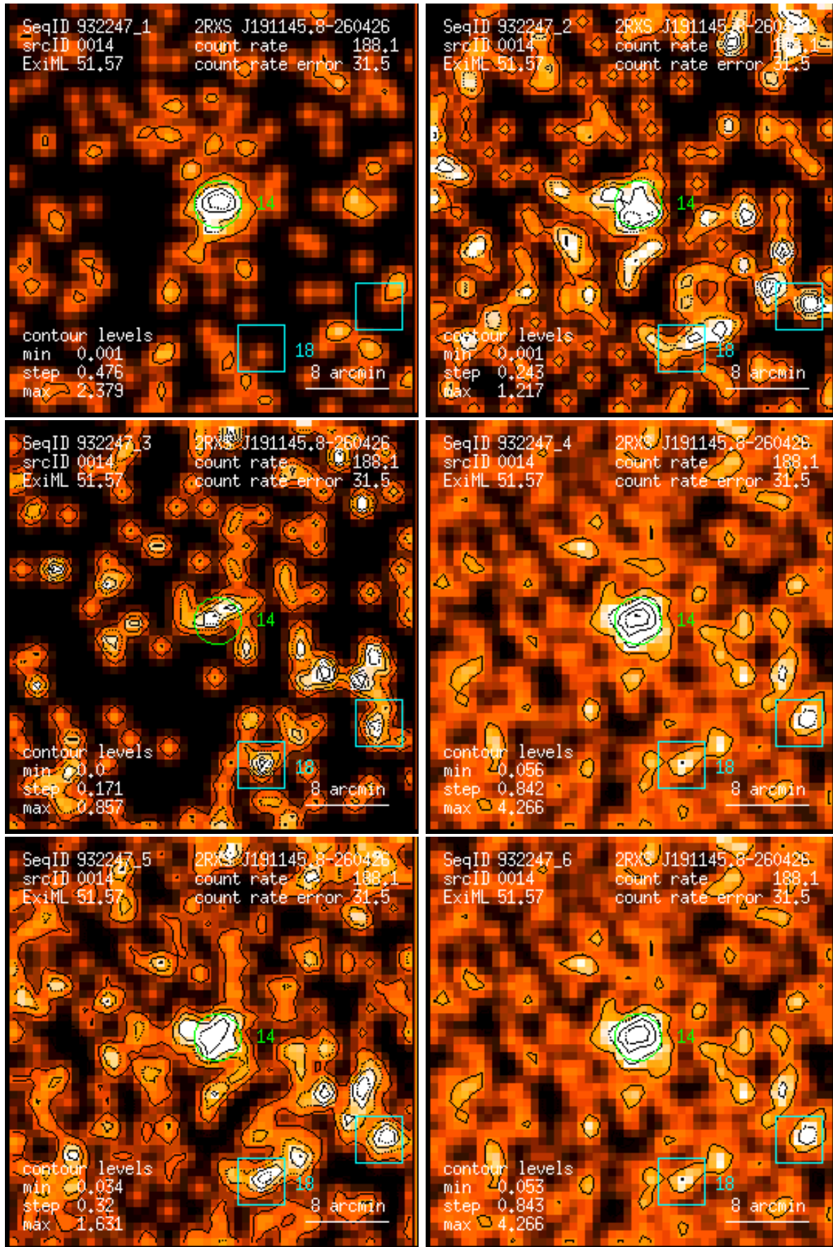
Figure 14: RASS 932247: detection 0014: band rate images, Gaussian filter: (1) PSPC channels 11 – 41, (2) 52 – 90, (3) 91 – 201, (4) 11 – 235, (5) 52 – 201, (6) 11 – 201. Broad band rates in counts/ks. Band rate contour levels in counts/ks/arcmin 2 .
