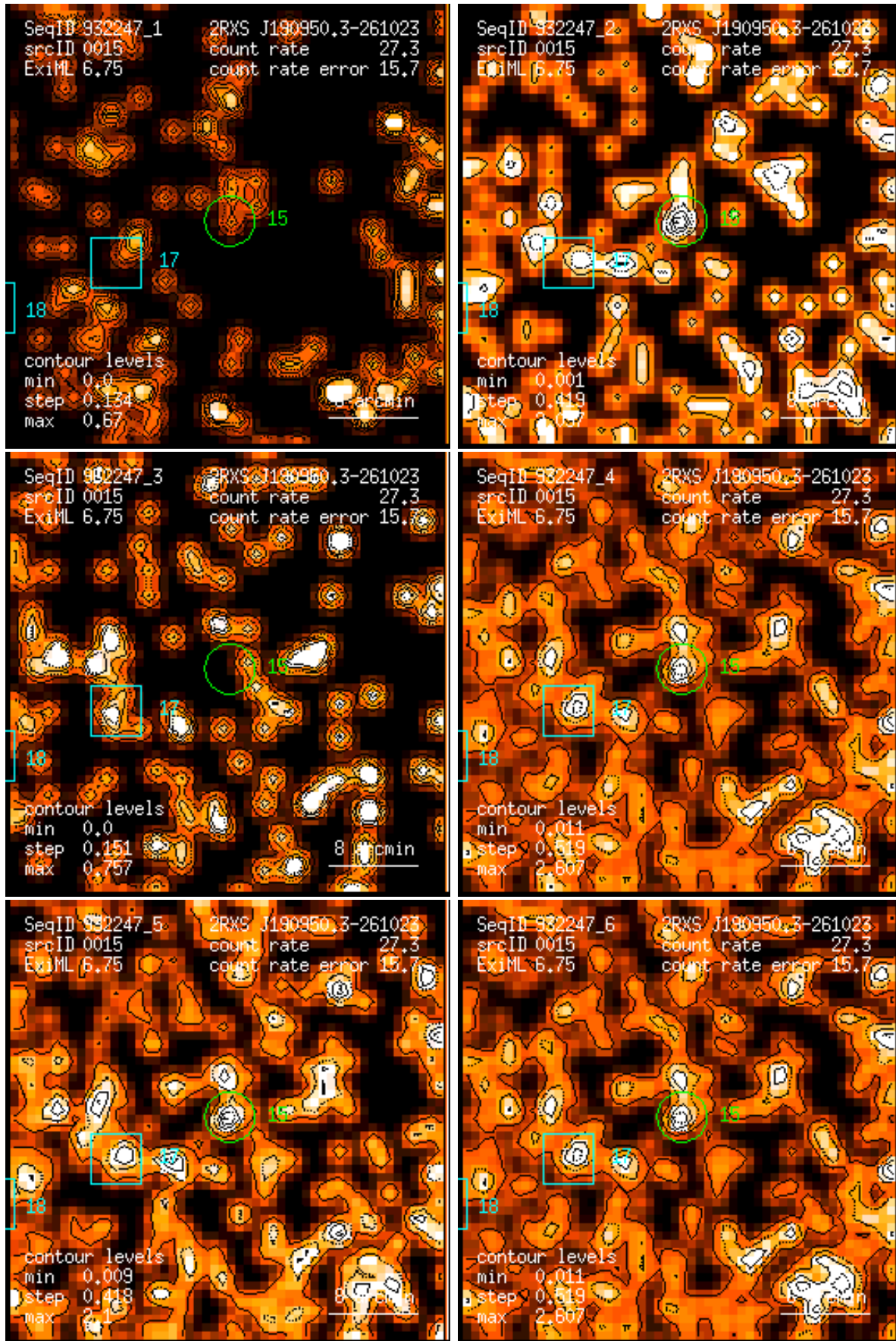
Figure 15: RASS 932247: detection 0015: band rate images, Gaussian filter: (1) PSPC channels 11 – 41, (2) 52 – 90, (3) 91 – 201, (4) 11 – 235, (5) 52 – 201, (6) 11 – 201. Broad band rates in counts/ks. Band rate contour levels in counts/ks/arcmin 2 .
