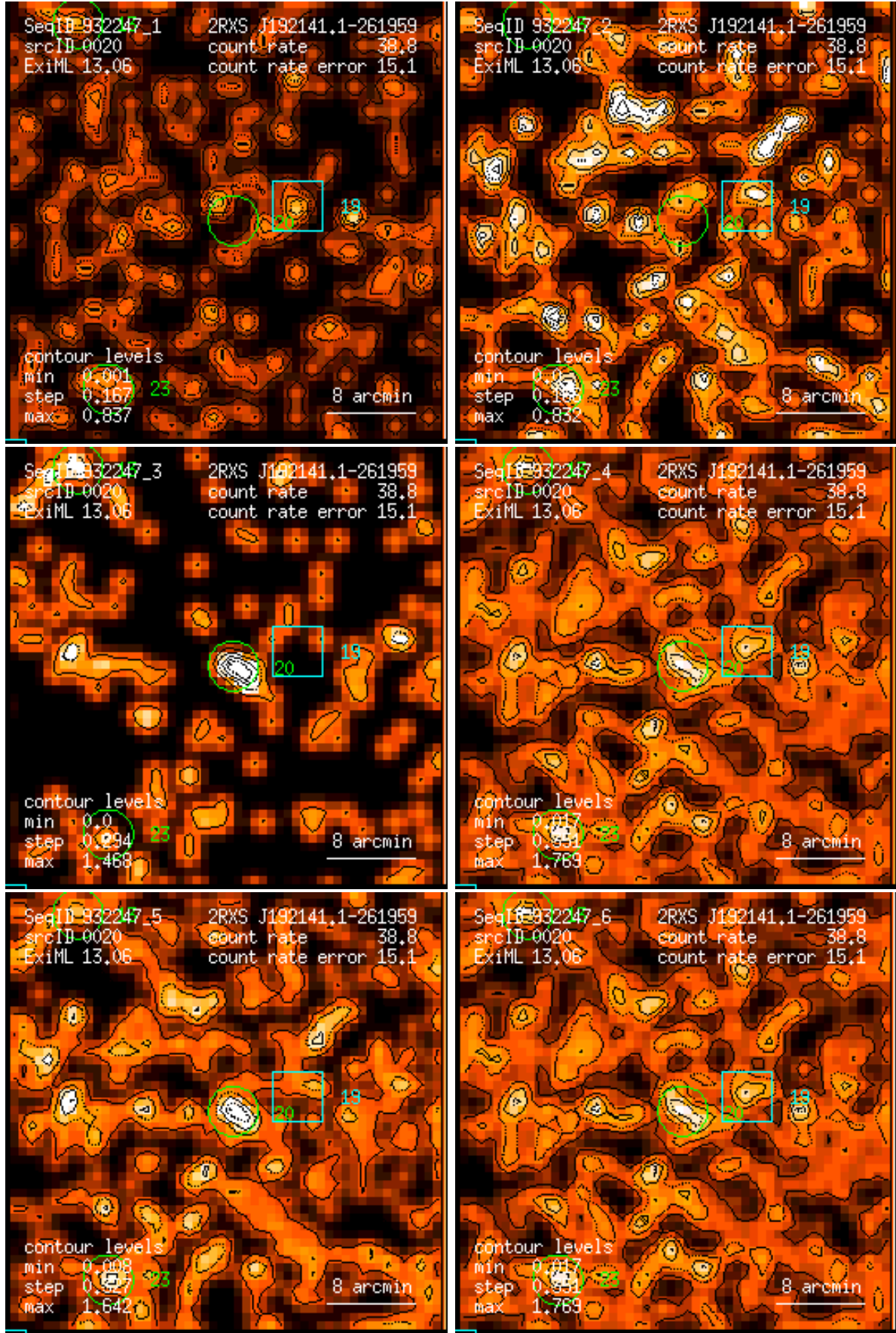
Figure 20: RASS 932247: detection 0020: band rate images, Gaussian filter: (1) PSPC channels 11 – 41, (2) 52 – 90, (3) 91 – 201, (4) 11 – 235, (5) 52 – 201, (6) 11 – 201. Broad band rates in counts/ks. Band rate contour levels in counts/ks/arcmin 2 .
