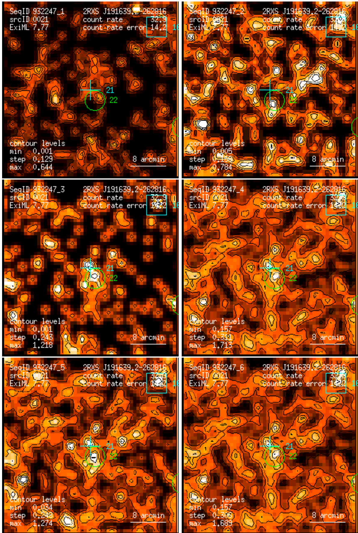
Figure 21: RASS 932247: detection 0021: band rate images, Gaussian filter: (1) PSPC channels 11 – 41, (2) 52 – 90, (3) 91 – 201, (4) 11 – 235, (5) 52 – 201, (6) 11 – 201. Broad band rates in counts/ks. Band rate contour levels in counts/ks/arcmin 2 .
