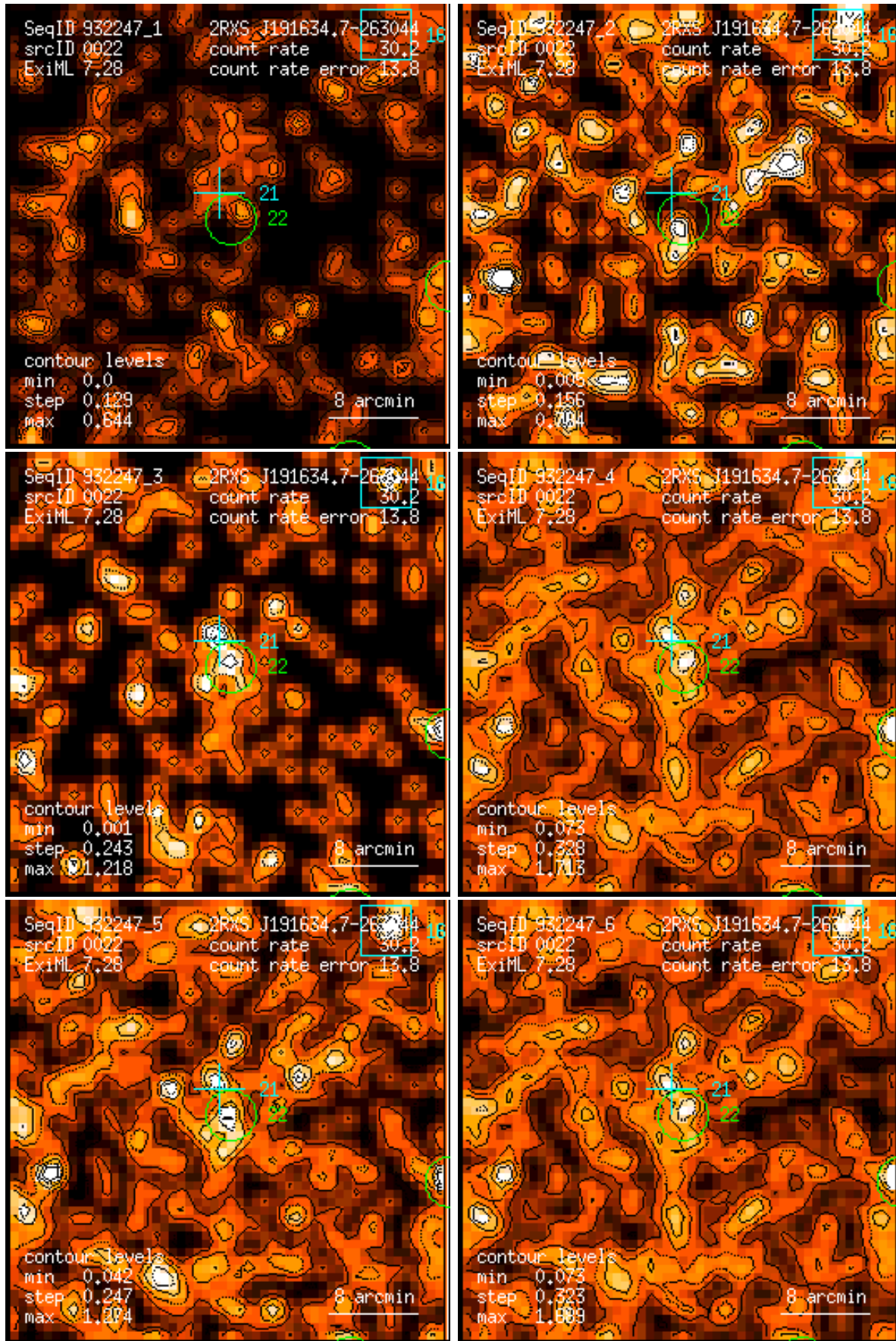
Figure 22: RASS 932247: detection 0022: band rate images, Gaussian filter: (1) PSPC channels 11 – 41, (2) 52 – 90, (3) 91 – 201, (4) 11 – 235, (5) 52 – 201, (6) 11 – 201. Broad band rates in counts/ks. Band rate contour levels in counts/ks/arcmin 2 .
