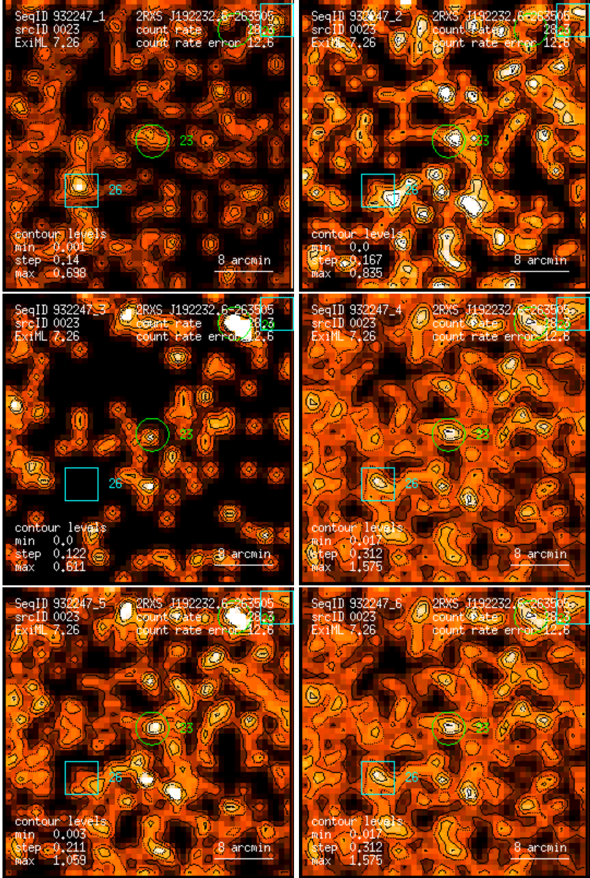
Figure 23: RASS 932247: detection 0023: band rate images, Gaussian filter: (1) PSPC channels 11 – 41, (2) 52 – 90, (3) 91 – 201, (4) 11 – 235, (5) 52 – 201, (6) 11 – 201. Broad band rates in counts/ks. Band rate contour levels in counts/ks/arcmin 2 .
