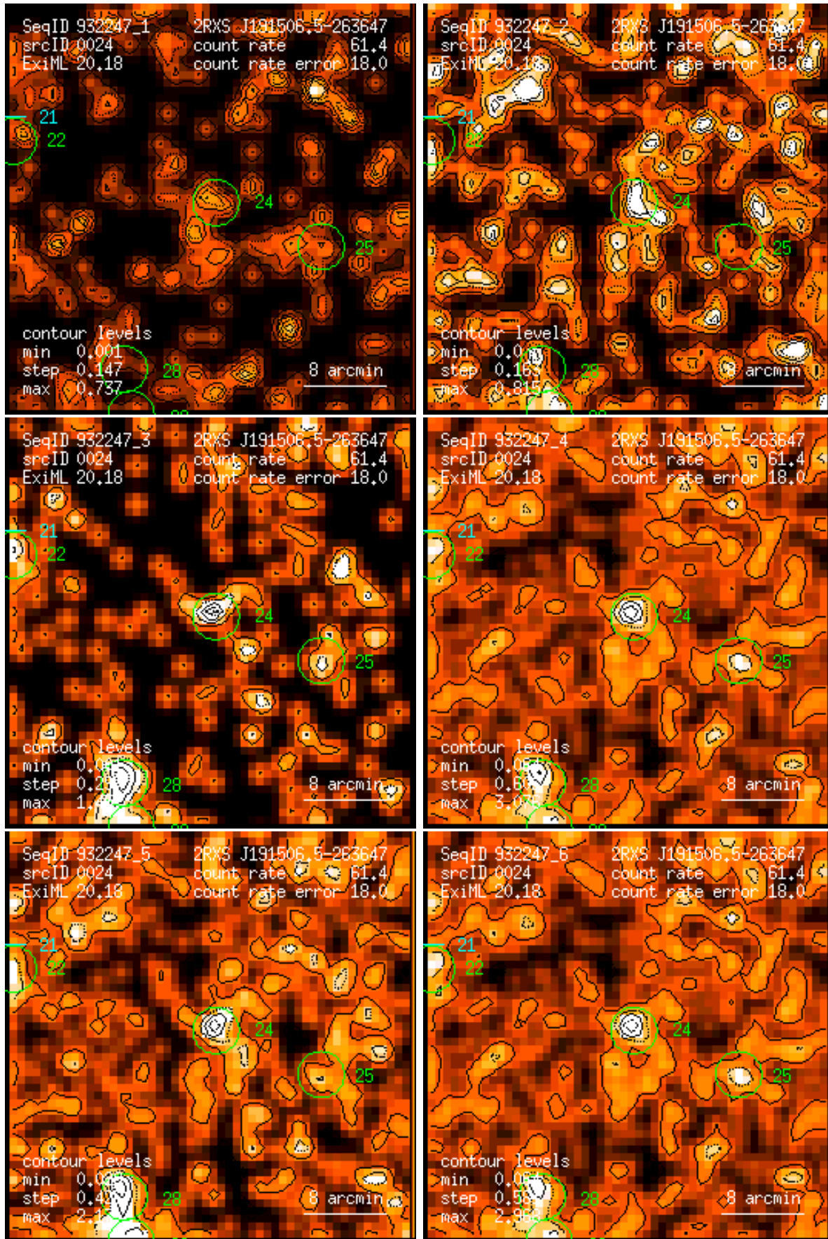
Figure 24: RASS 932247: detection 0024: band rate images, Gaussian filter: (1) PSPC channels 11 – 41, (2) 52 – 90, (3) 91 – 201, (4) 11 – 235, (5) 52 – 201, (6) 11 – 201. Broad band rates in counts/ks. Band rate contour levels in counts/ks/arcmin 2 .
