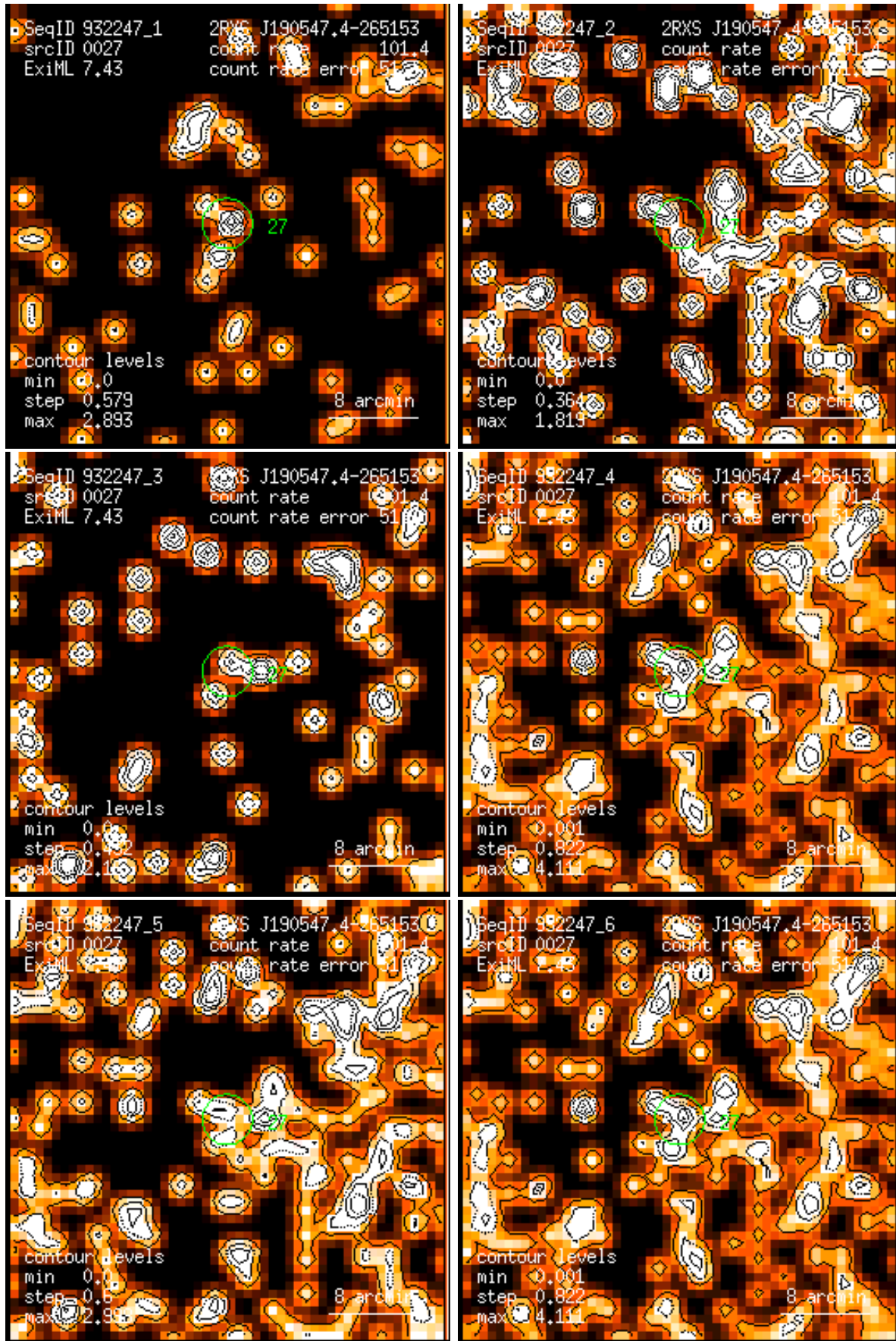
Figure 27: RASS 932247: detection 0027: band rate images, Gaussian filter: (1) PSPC channels 11 – 41, (2) 52 – 90, (3) 91 – 201, (4) 11 – 235, (5) 52 – 201, (6) 11 – 201. Broad band rates in counts/ks. Band rate contour levels in counts/ks/arcmin 2 .
