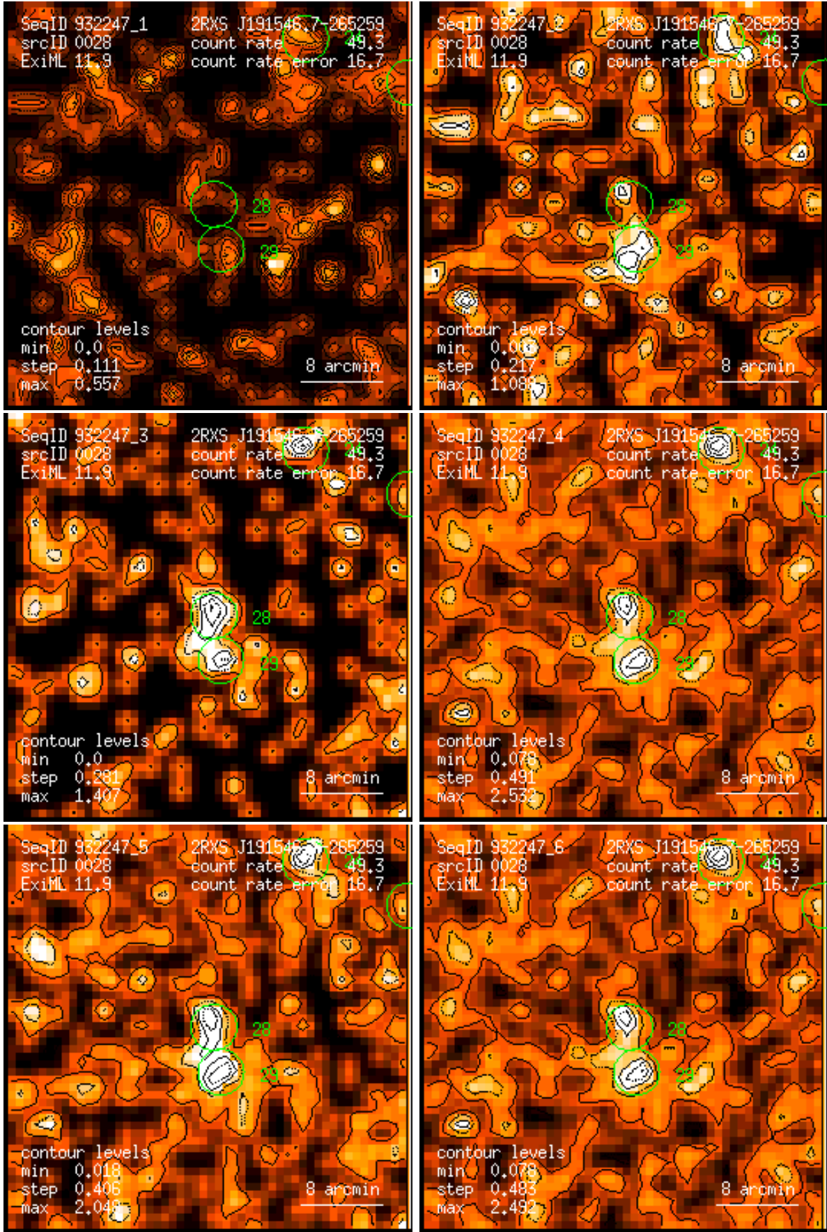
Figure 28: RASS 932247: detection 0028: band rate images, Gaussian filter: (1) PSPC channels 11 – 41, (2) 52 – 90, (3) 91 – 201, (4) 11 – 235, (5) 52 – 201, (6) 11 – 201. Broad band rates in counts/ks. Band rate contour levels in counts/ks/arcmin 2 .
