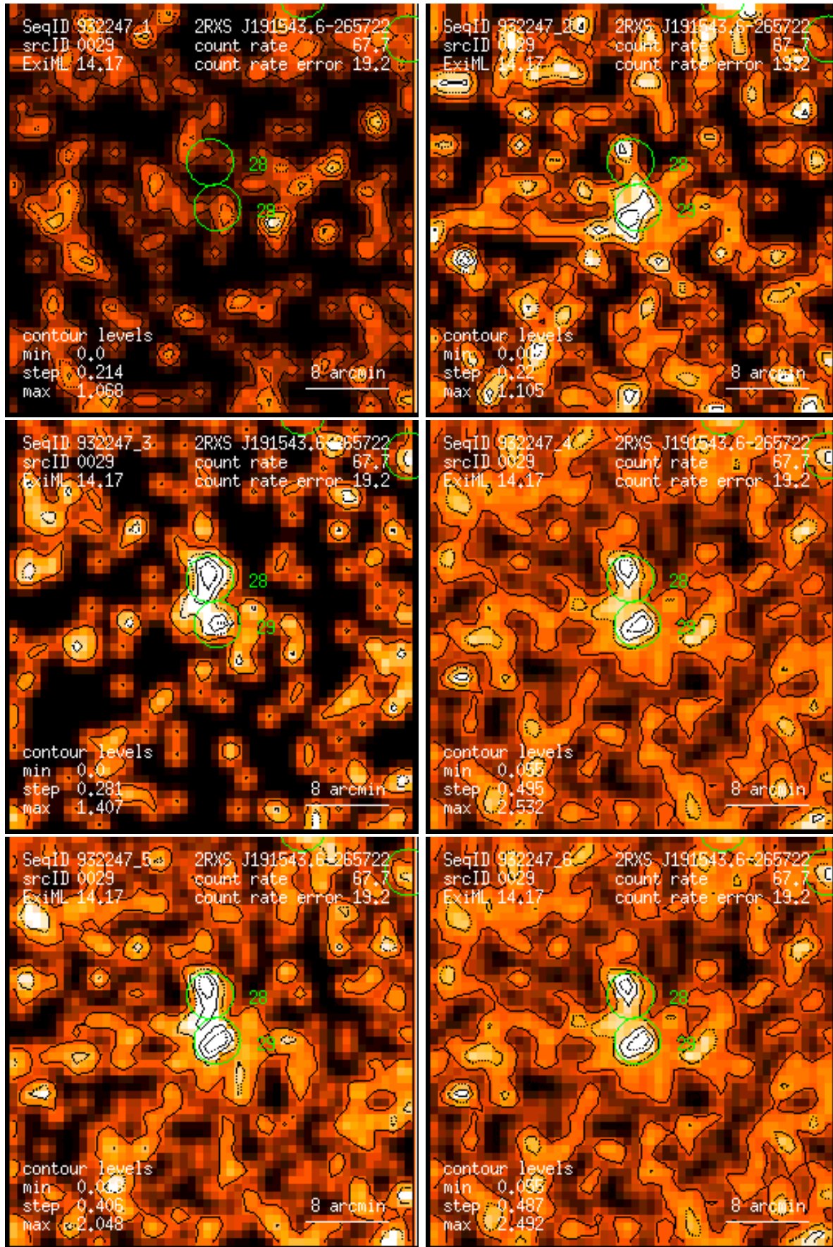
Figure 29: RASS 932247: detection 0029: band rate images, Gaussian filter: (1) PSPC channels 11 – 41, (2) 52 – 90, (3) 91 – 201, (4) 11 – 235, (5) 52 – 201, (6) 11 – 201. Broad band rates in counts/ks. Band rate contour levels in counts/ks/arcmin 2 .
