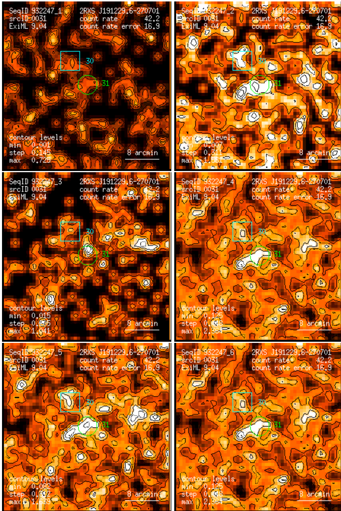
Figure 31: RASS 932247: detection 0031: band rate images, Gaussian filter: (1) PSPC channels 11 – 41, (2) 52 – 90, (3) 91 – 201, (4) 11 – 235, (5) 52 – 201, (6) 11 – 201. Broad band rates in counts/ks. Band rate contour levels in counts/ks/arcmin 2 .
