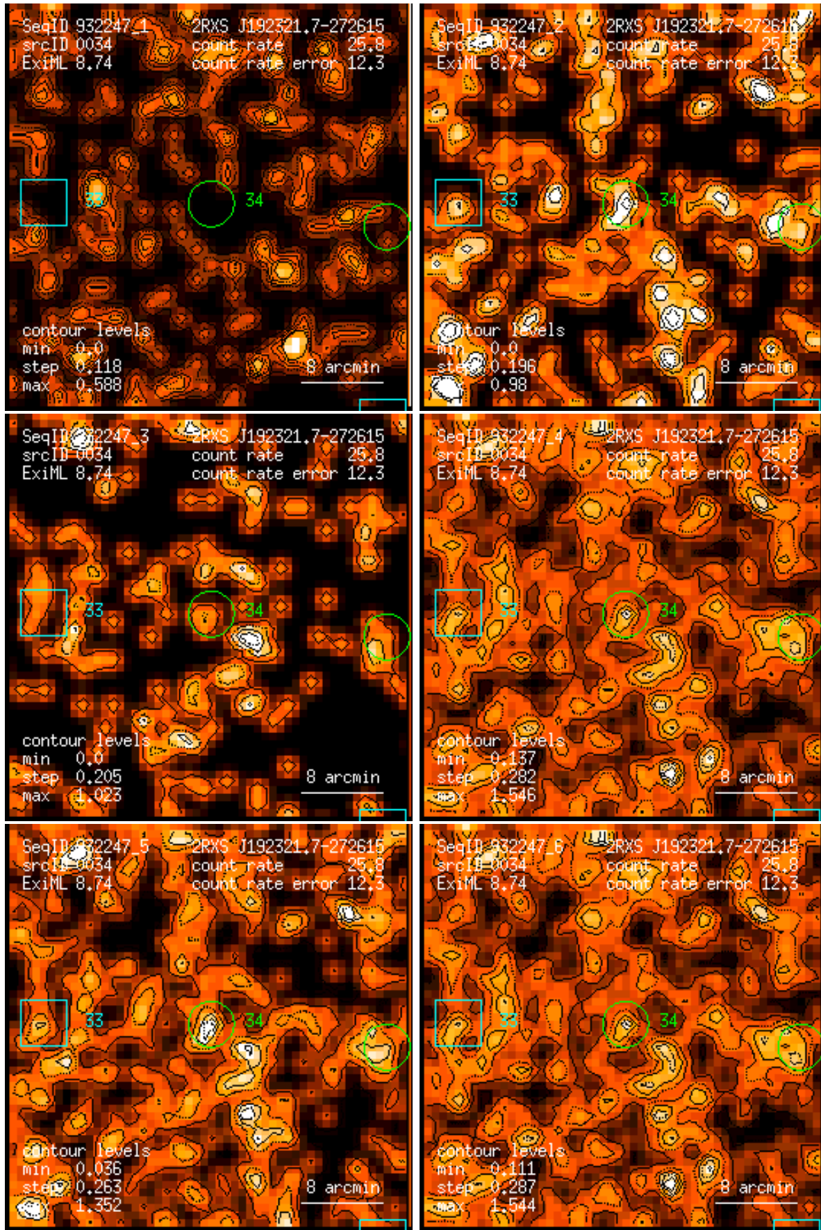
Figure 34: RASS 932247: detection 0034: band rate images, Gaussian filter: (1) PSPC channels 11 – 41, (2) 52 – 90, (3) 91 – 201, (4) 11 – 235, (5) 52 – 201, (6) 11 – 201. Broad band rates in counts/ks. Band rate contour levels in counts/ks/arcmin 2 .
