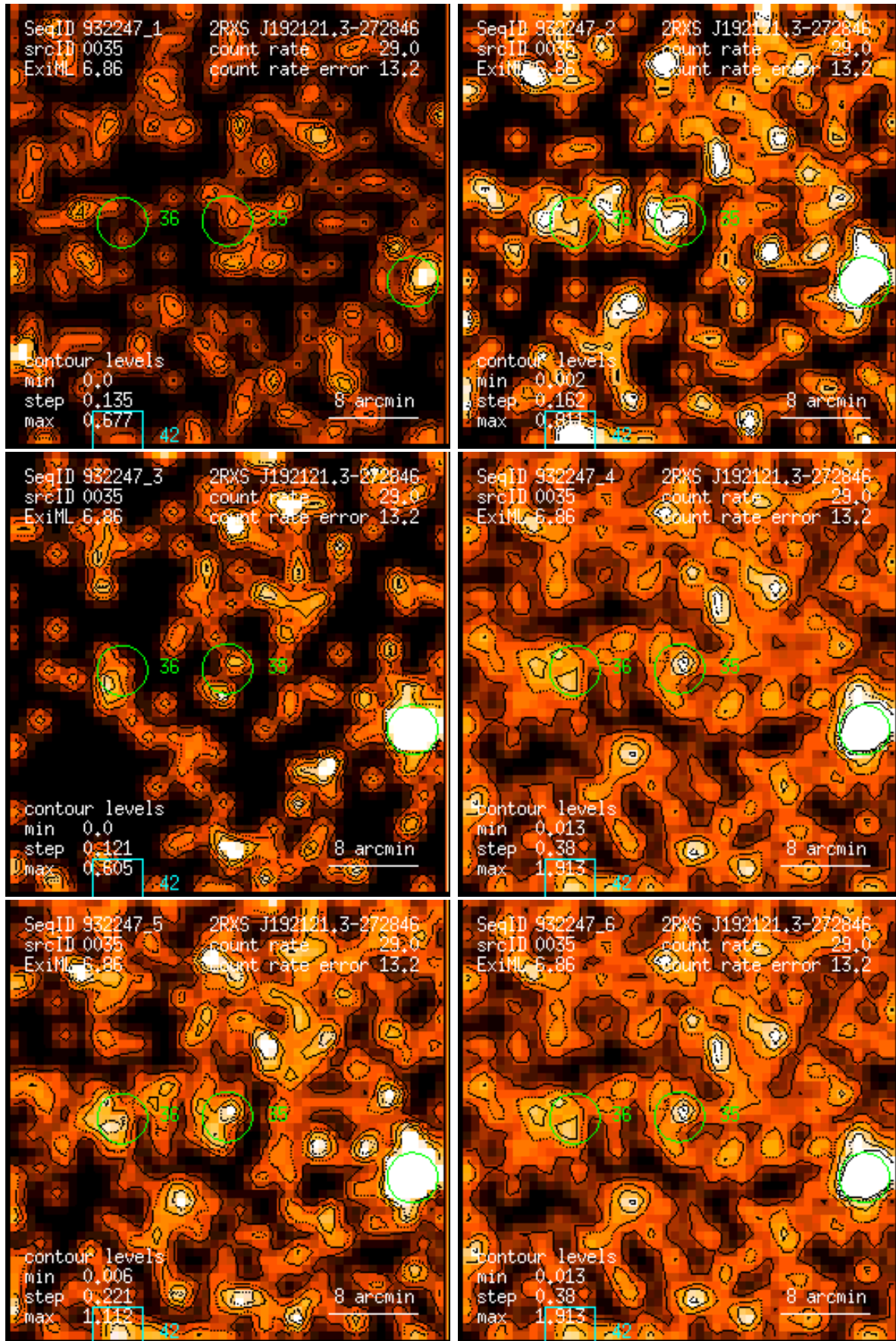
Figure 35: RASS 932247: detection 0035: band rate images, Gaussian filter: (1) PSPC channels 11 – 41, (2) 52 – 90, (3) 91 – 201, (4) 11 – 235, (5) 52 – 201, (6) 11 – 201. Broad band rates in counts/ks. Band rate contour levels in counts/ks/arcmin 2 .
