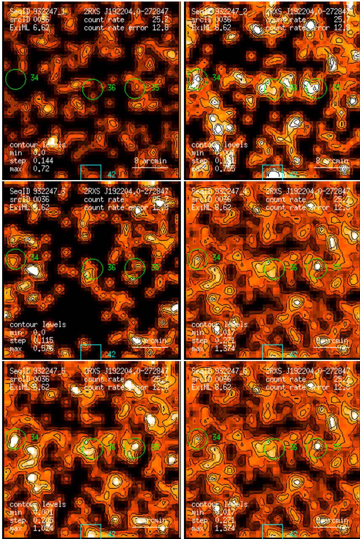
Figure 36: RASS 932247: detection 0036: band rate images, Gaussian filter: (1) PSPC channels 11 – 41, (2) 52 – 90, (3) 91 – 201, (4) 11 – 235, (5) 52 – 201, (6) 11 – 201. Broad band rates in counts/ks. Band rate contour levels in counts/ks/arcmin 2 .
