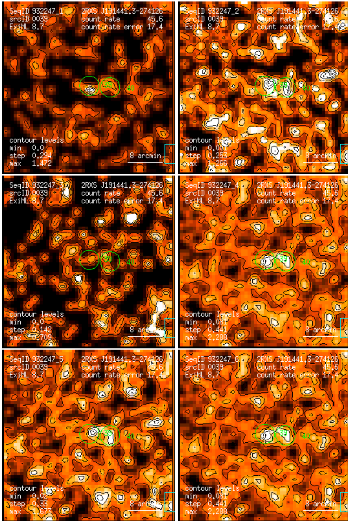
Figure 39: RASS 932247: detection 0039: band rate images, Gaussian filter: (1) PSPC channels 11 – 41, (2) 52 – 90, (3) 91 – 201, (4) 11 – 235, (5) 52 – 201, (6) 11 – 201. Broad band rates in counts/ks. Band rate contour levels in counts/ks/arcmin 2 .
