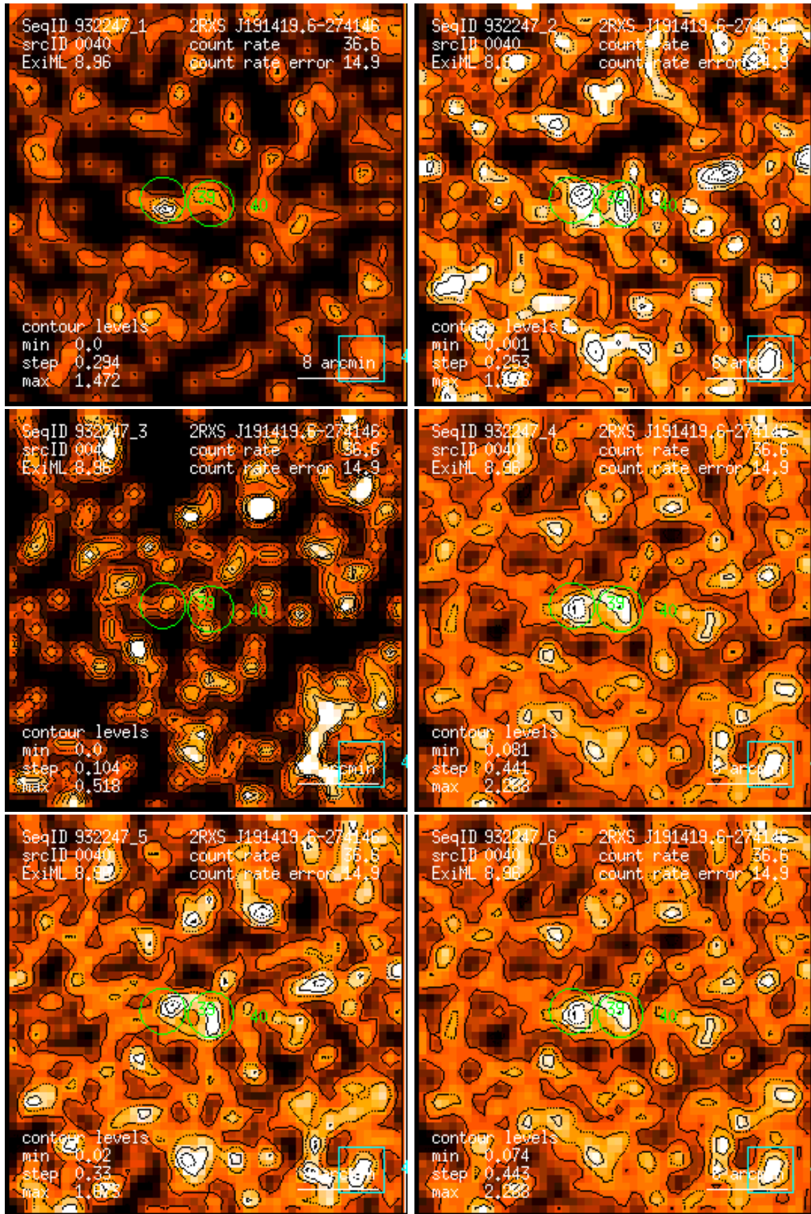
Figure 40: RASS 932247: detection 0040: band rate images, Gaussian filter: (1) PSPC channels 11 – 41, (2) 52 – 90, (3) 91 – 201, (4) 11 – 235, (5) 52 – 201, (6) 11 – 201. Broad band rates in counts/ks. Band rate contour levels in counts/ks/arcmin 2 .
