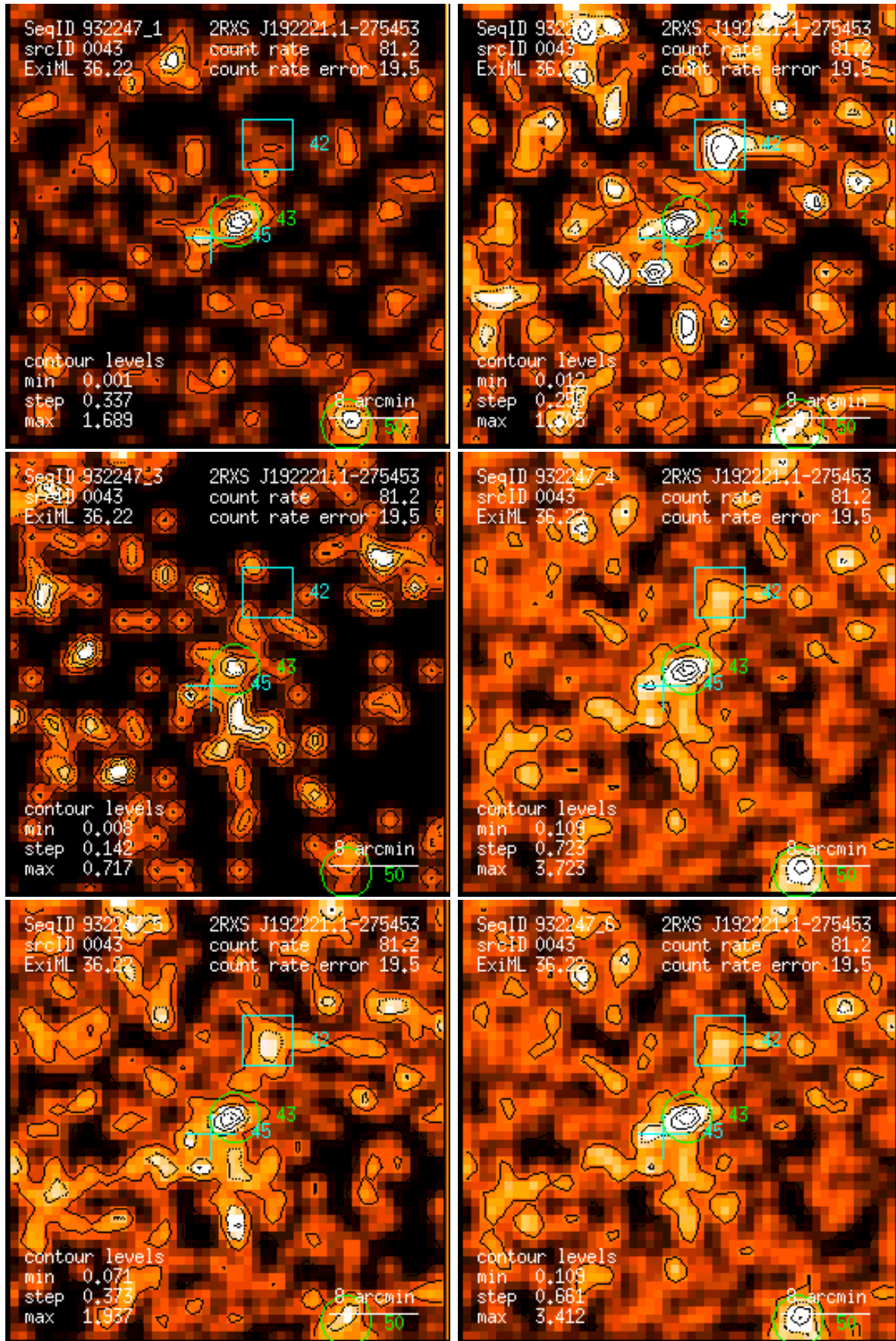
Figure 43: RASS 932247: detection 0043: band rate images, Gaussian filter: (1) PSPC channels 11 – 41, (2) 52 – 90, (3) 91 – 201, (4) 11 – 235, (5) 52 – 201, (6) 11 – 201. Broad band rates in counts/ks. Band rate contour levels in counts/ks/arcmin 2 .
