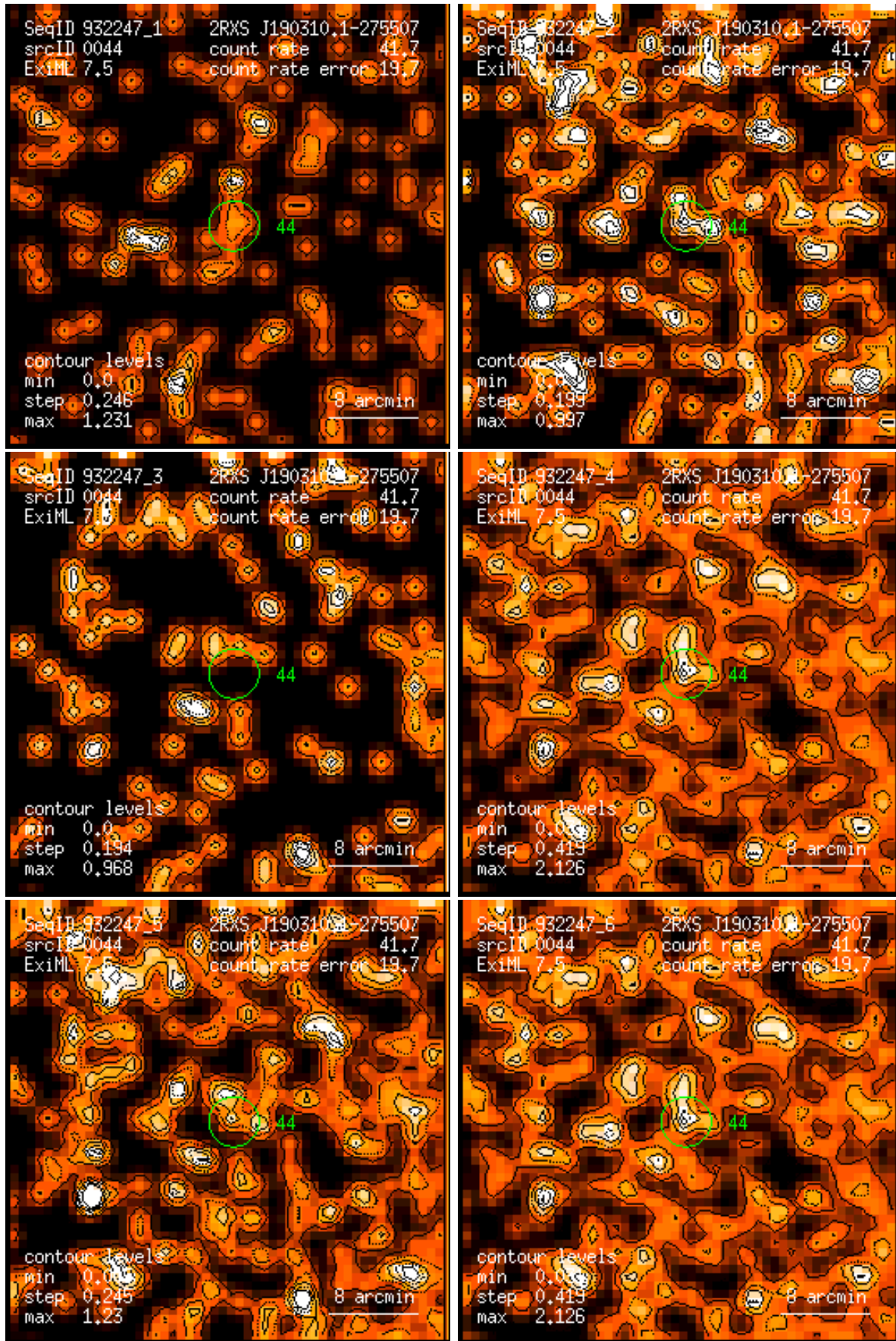
Figure 44: RASS 932247: detection 0044: band rate images, Gaussian filter: (1) PSPC channels 11 – 41, (2) 52 – 90, (3) 91 – 201, (4) 11 – 235, (5) 52 – 201, (6) 11 – 201. Broad band rates in counts/ks. Band rate contour levels in counts/ks/arcmin 2 .
