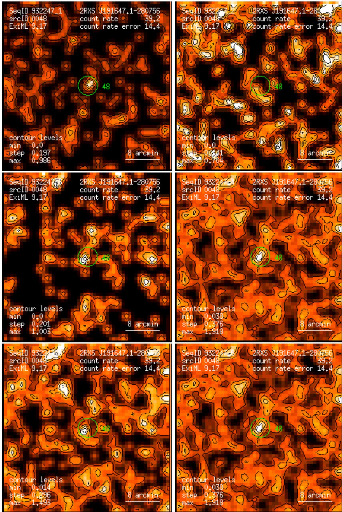
Figure 48: RASS 932247: detection 0048: band rate images, Gaussian filter: (1) PSPC channels 11 – 41, (2) 52 – 90, (3) 91 – 201, (4) 11 – 235, (5) 52 – 201, (6) 11 – 201. Broad band rates in counts/ks. Band rate contour levels in counts/ks/arcmin 2 .
