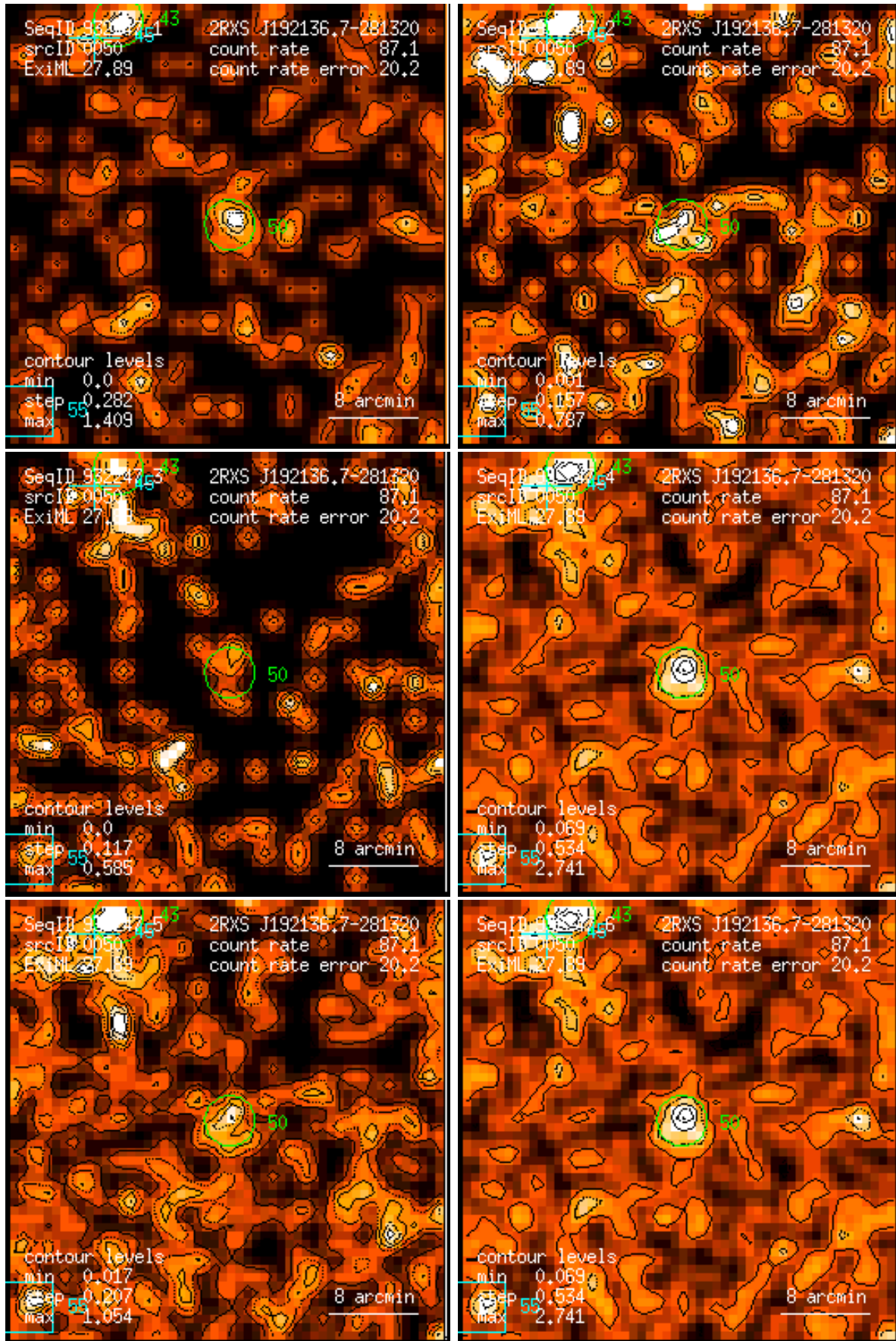
Figure 50: RASS 932247: detection 0050: band rate images, Gaussian filter: (1) PSPC channels 11 – 41, (2) 52 – 90, (3) 91 – 201, (4) 11 – 235, (5) 52 – 201, (6) 11 – 201. Broad band rates in counts/ks. Band rate contour levels in counts/ks/arcmin 2 .
