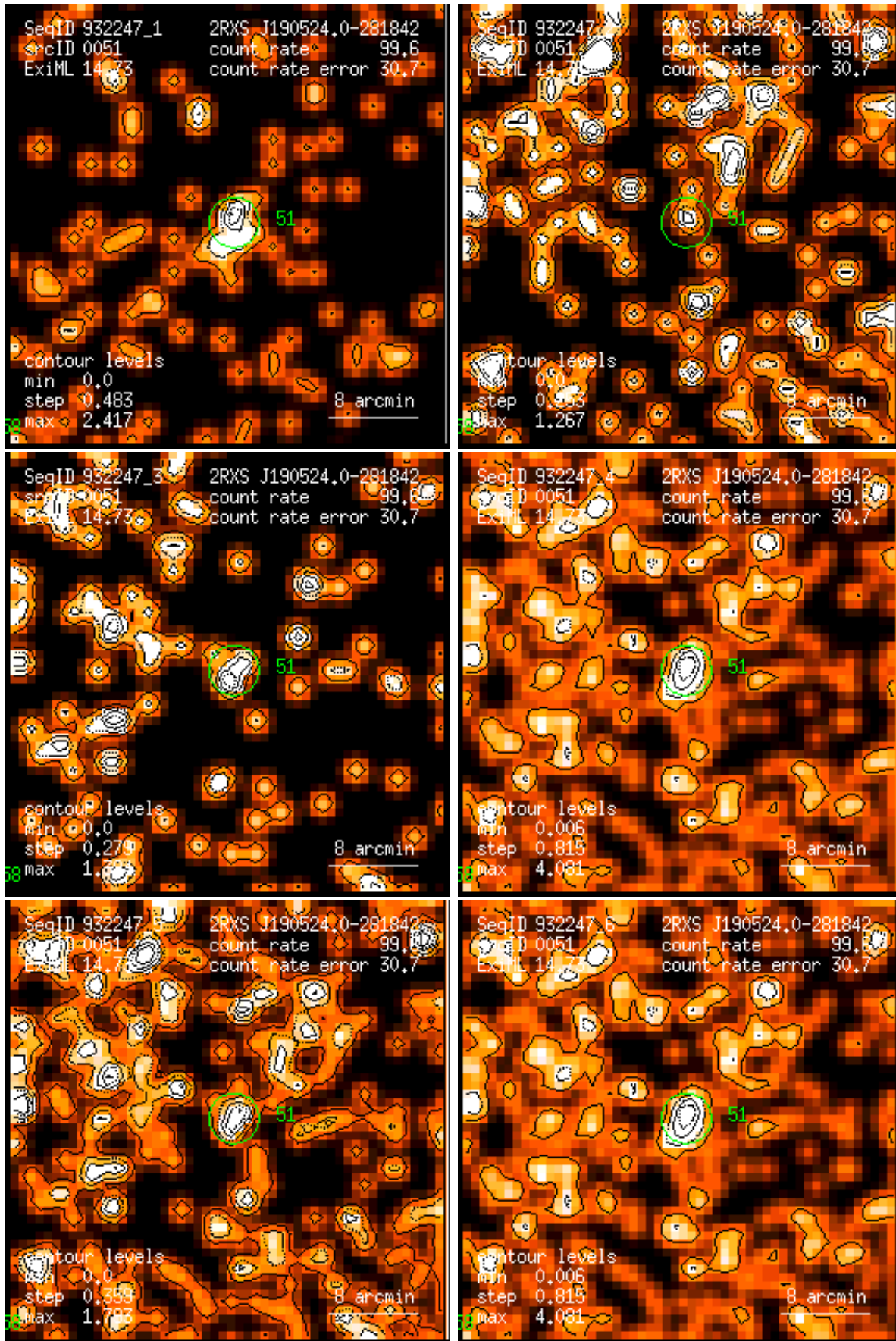
Figure 51: RASS 932247: detection 0051: band rate images, Gaussian filter: (1) PSPC channels 11 – 41, (2) 52 – 90, (3) 91 – 201, (4) 11 – 235, (5) 52 – 201, (6) 11 – 201. Broad band rates in counts/ks. Band rate contour levels in counts/ks/arcmin 2 .
