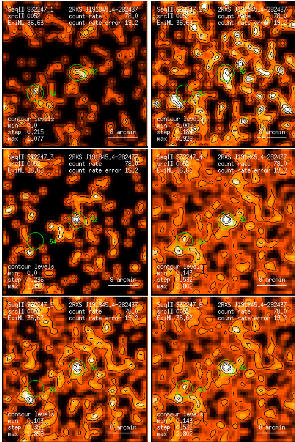
Figure 52: RASS 932247: detection 0052: band rate images, Gaussian filter: (1) PSPC channels 11 – 41, (2) 52 – 90, (3) 91 – 201, (4) 11 – 235, (5) 52 – 201, (6) 11 – 201. Broad band rates in counts/ks. Band rate contour levels in counts/ks/arcmin 2 .
