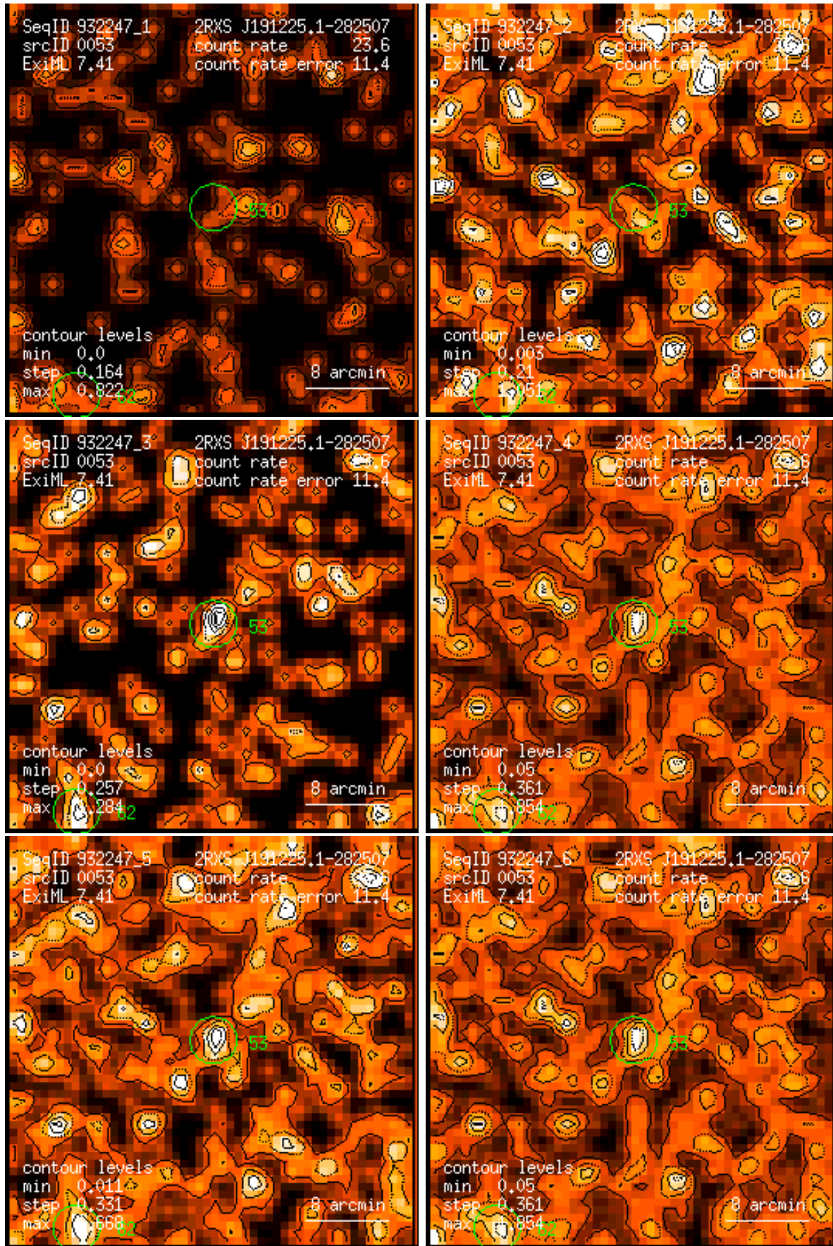
Figure 53: RASS 932247: detection 0053: band rate images, Gaussian filter: (1) PSPC channels 11 – 41, (2) 52 – 90, (3) 91 – 201, (4) 11 – 235, (5) 52 – 201, (6) 11 – 201. Broad band rates in counts/ks. Band rate contour levels in counts/ks/arcmin 2 .
