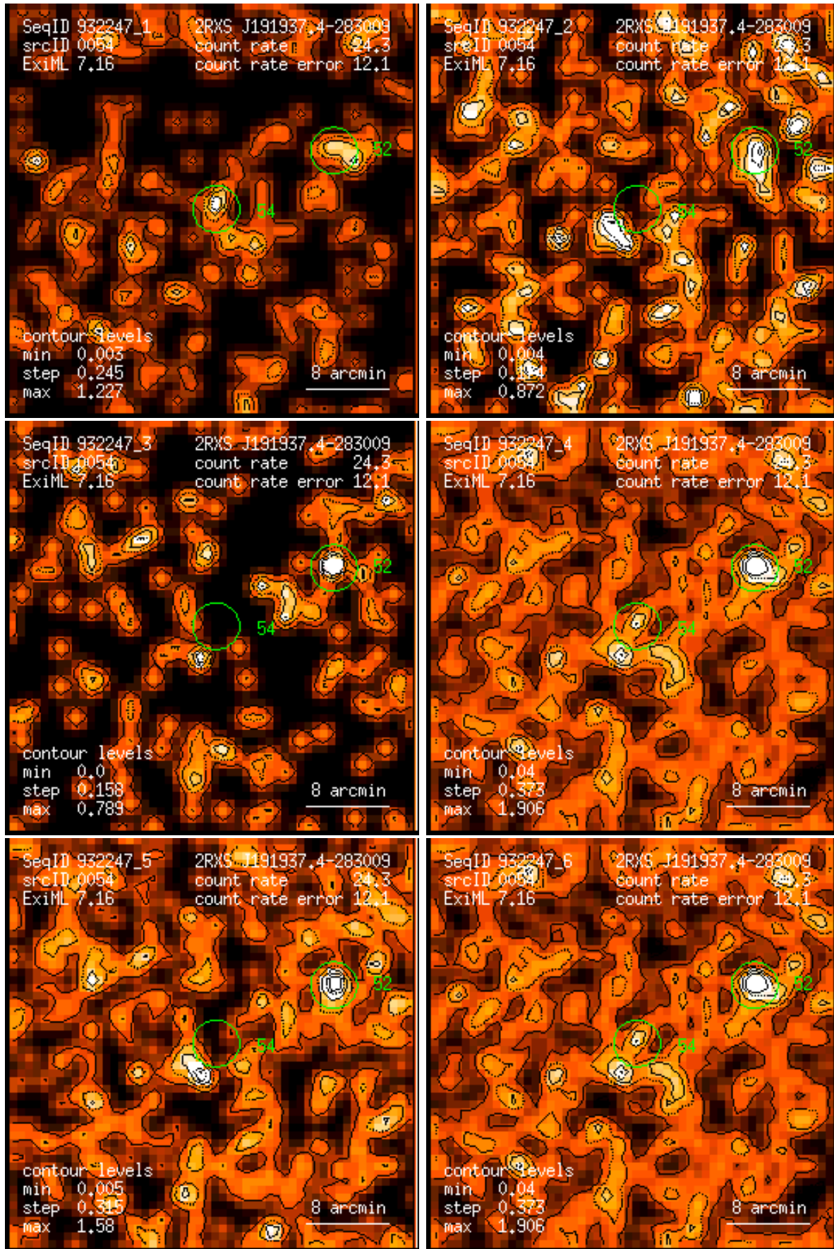
Figure 54: RASS 932247: detection 0054: band rate images, Gaussian filter: (1) PSPC channels 11 – 41, (2) 52 – 90, (3) 91 – 201, (4) 11 – 235, (5) 52 – 201, (6) 11 – 201. Broad band rates in counts/ks. Band rate contour levels in counts/ks/arcmin 2 .
