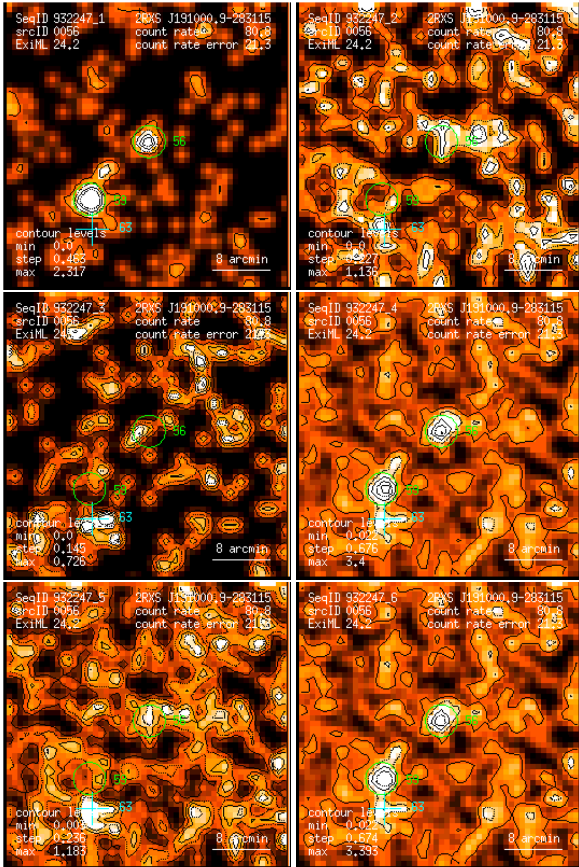
Figure 56: RASS 932247: detection 0056: band rate images, Gaussian filter: (1) PSPC channels 11 – 41, (2) 52 – 90, (3) 91 – 201, (4) 11 – 235, (5) 52 – 201, (6) 11 – 201. Broad band rates in counts/ks. Band rate contour levels in counts/ks/arcmin 2 .
