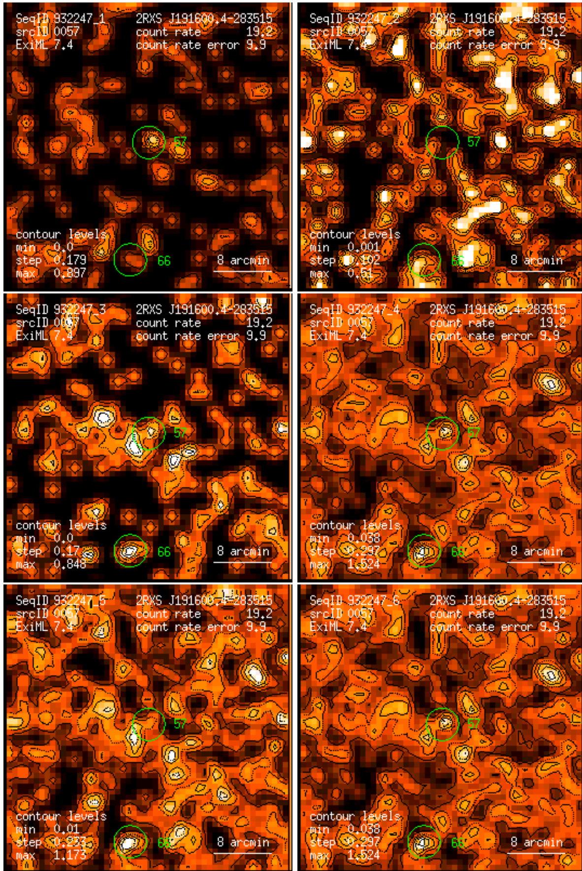
Figure 57: RASS 932247: detection 0057: band rate images, Gaussian filter: (1) PSPC channels 11 – 41, (2) 52 – 90, (3) 91 – 201, (4) 11 – 235, (5) 52 – 201, (6) 11 – 201. Broad band rates in counts/ks. Band rate contour levels in counts/ks/arcmin 2 .
