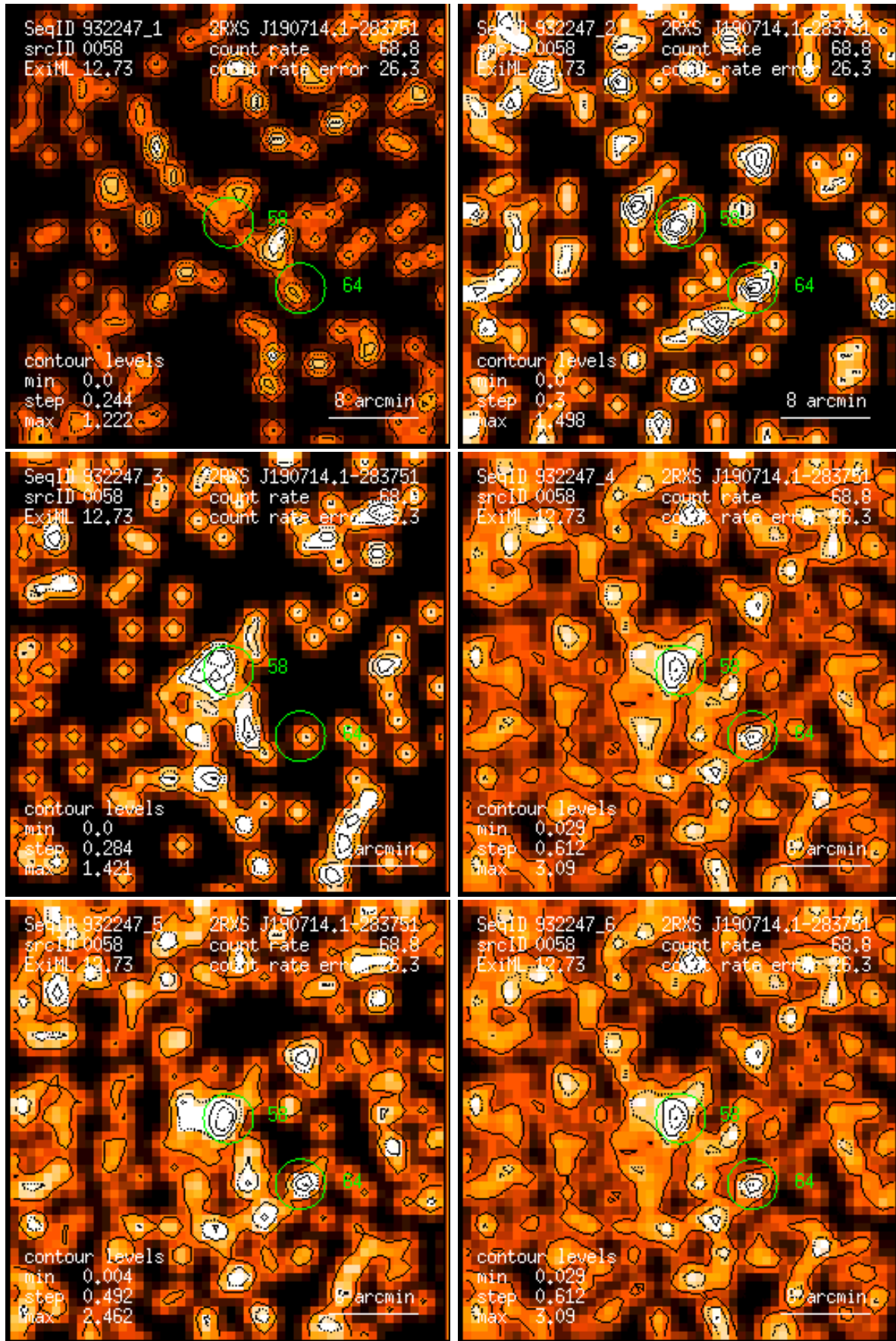
Figure 58: RASS 932247: detection 0058: band rate images, Gaussian filter: (1) PSPC channels 11 – 41, (2) 52 – 90, (3) 91 – 201, (4) 11 – 235, (5) 52 – 201, (6) 11 – 201. Broad band rates in counts/ks. Band rate contour levels in counts/ks/arcmin 2 .
