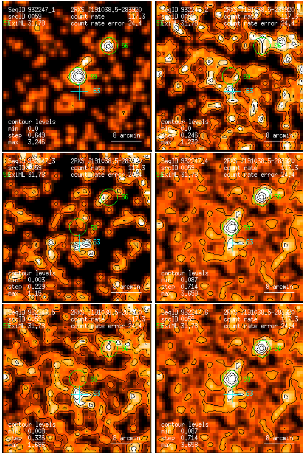
Figure 59: RASS 932247: detection 0059: band rate images, Gaussian filter: (1) PSPC channels 11 – 41, (2) 52 – 90, (3) 91 – 201, (4) 11 – 235, (5) 52 – 201, (6) 11 – 201. Broad band rates in counts/ks. Band rate contour levels in counts/ks/arcmin 2 .
