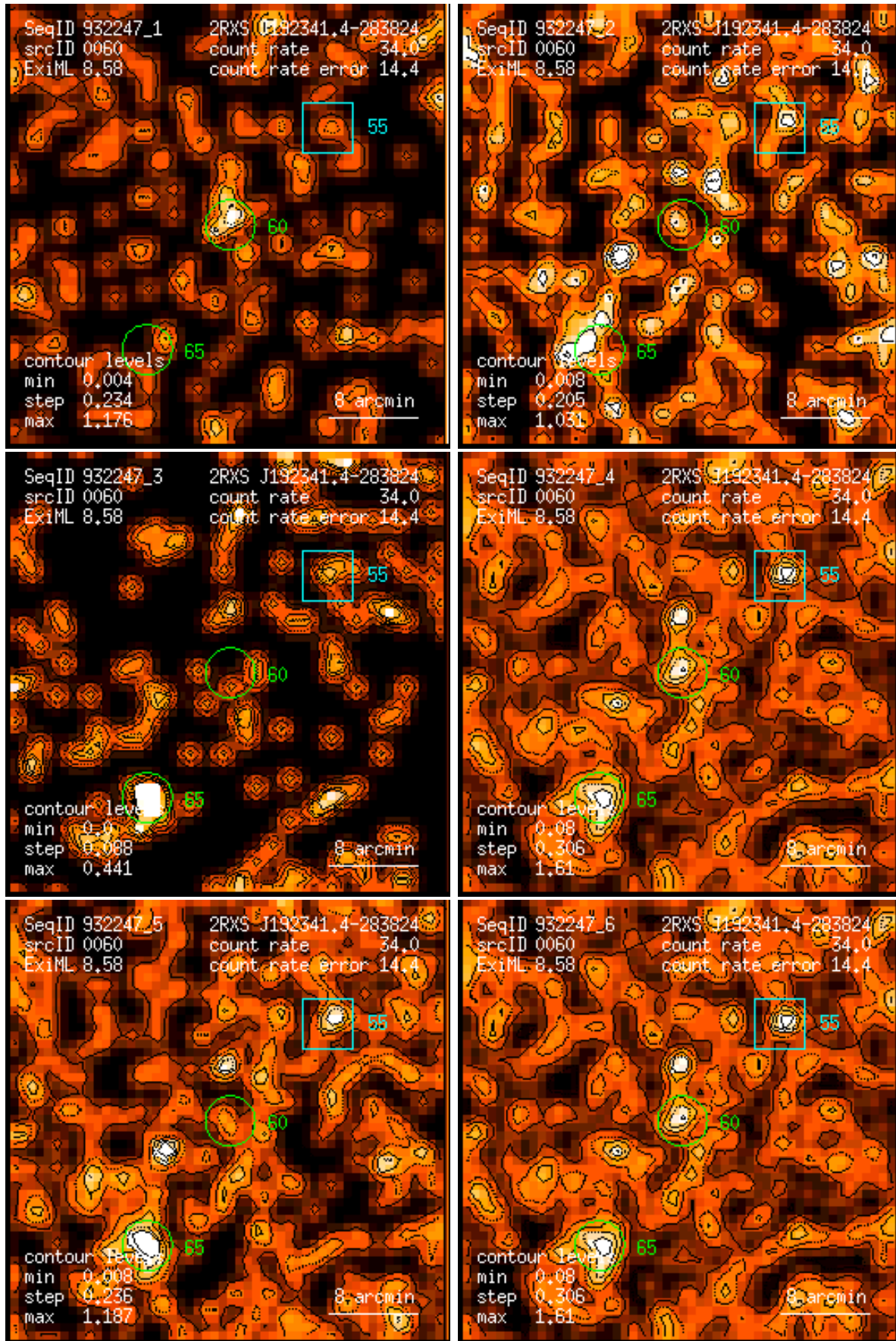
Figure 60: RASS 932247: detection 0060: band rate images, Gaussian filter: (1) PSPC channels 11 – 41, (2) 52 – 90, (3) 91 – 201, (4) 11 – 235, (5) 52 – 201, (6) 11 – 201. Broad band rates in counts/ks. Band rate contour levels in counts/ks/arcmin 2 .
