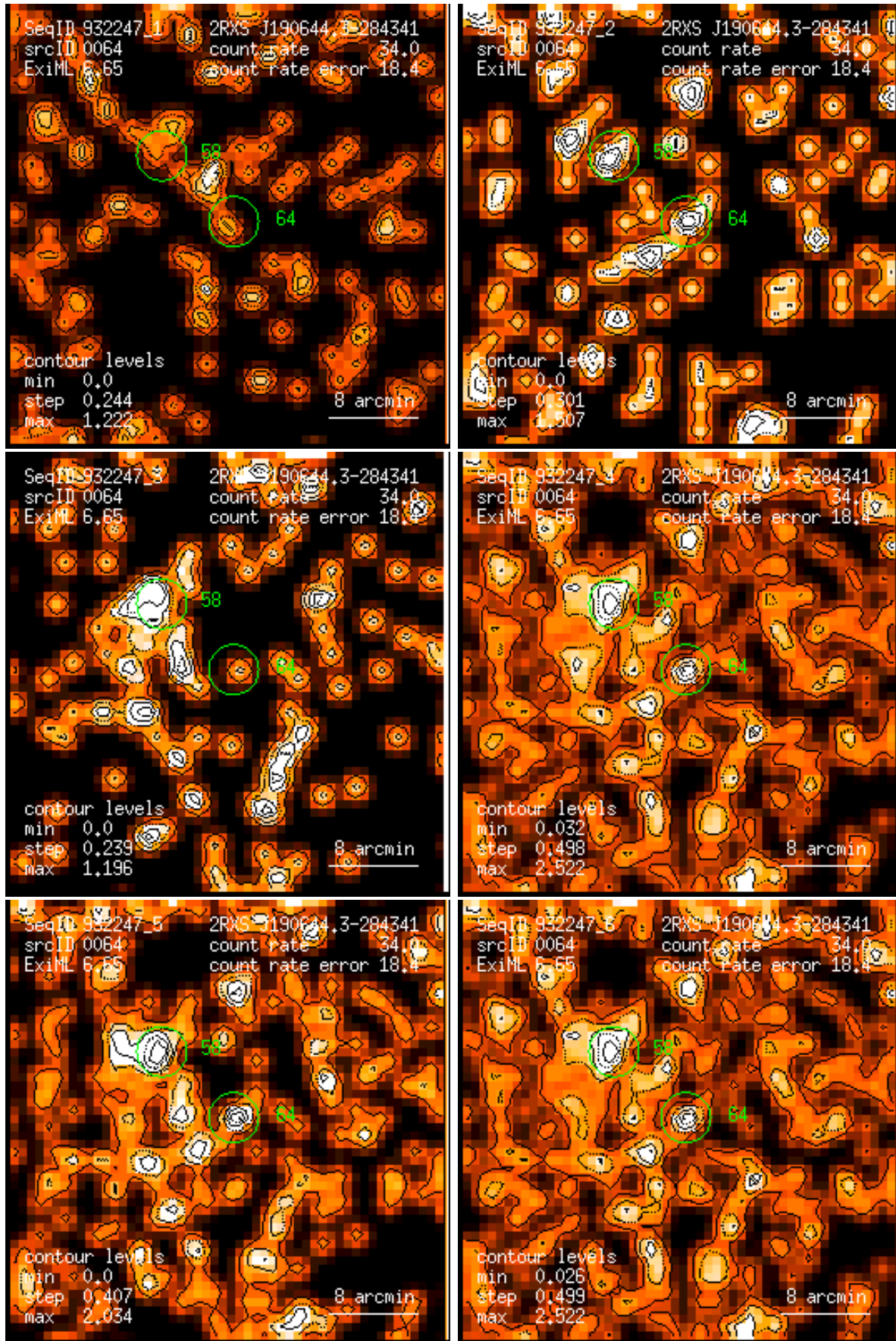
Figure 64: RASS 932247: detection 0064: band rate images, Gaussian filter: (1) PSPC channels 11 – 41, (2) 52 – 90, (3) 91 – 201, (4) 11 – 235, (5) 52 – 201, (6) 11 – 201. Broad band rates in counts/ks. Band rate contour levels in counts/ks/arcmin 2 .
