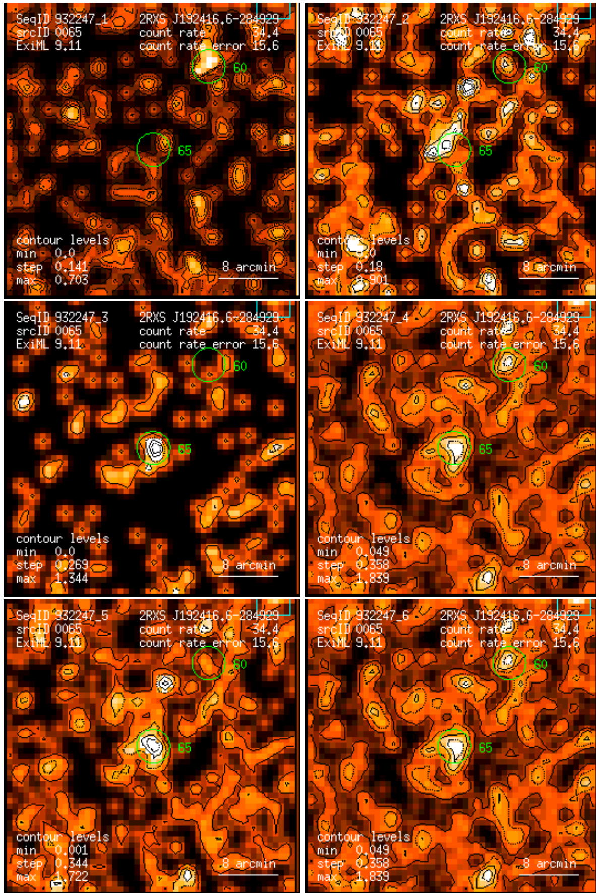
Figure 65: RASS 932247: detection 0065: band rate images, Gaussian filter: (1) PSPC channels 11 – 41, (2) 52 – 90, (3) 91 – 201, (4) 11 – 235, (5) 52 – 201, (6) 11 – 201. Broad band rates in counts/ks. Band rate contour levels in counts/ks/arcmin 2 .
