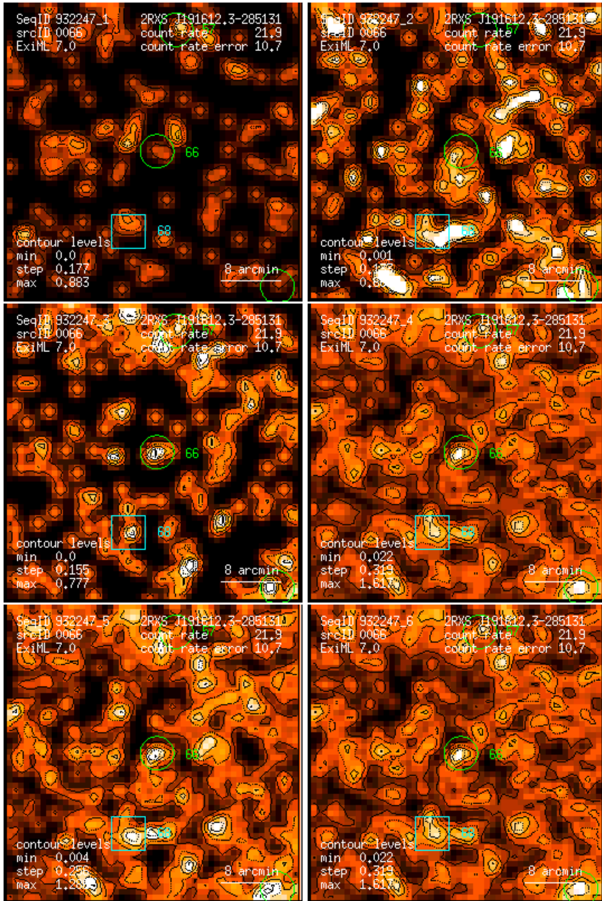
Figure 66: RASS 932247: detection 0066: band rate images, Gaussian filter: (1) PSPC channels 11 – 41, (2) 52 – 90, (3) 91 – 201, (4) 11 – 235, (5) 52 – 201, (6) 11 – 201. Broad band rates in counts/ks. Band rate contour levels in counts/ks/arcmin 2 .
