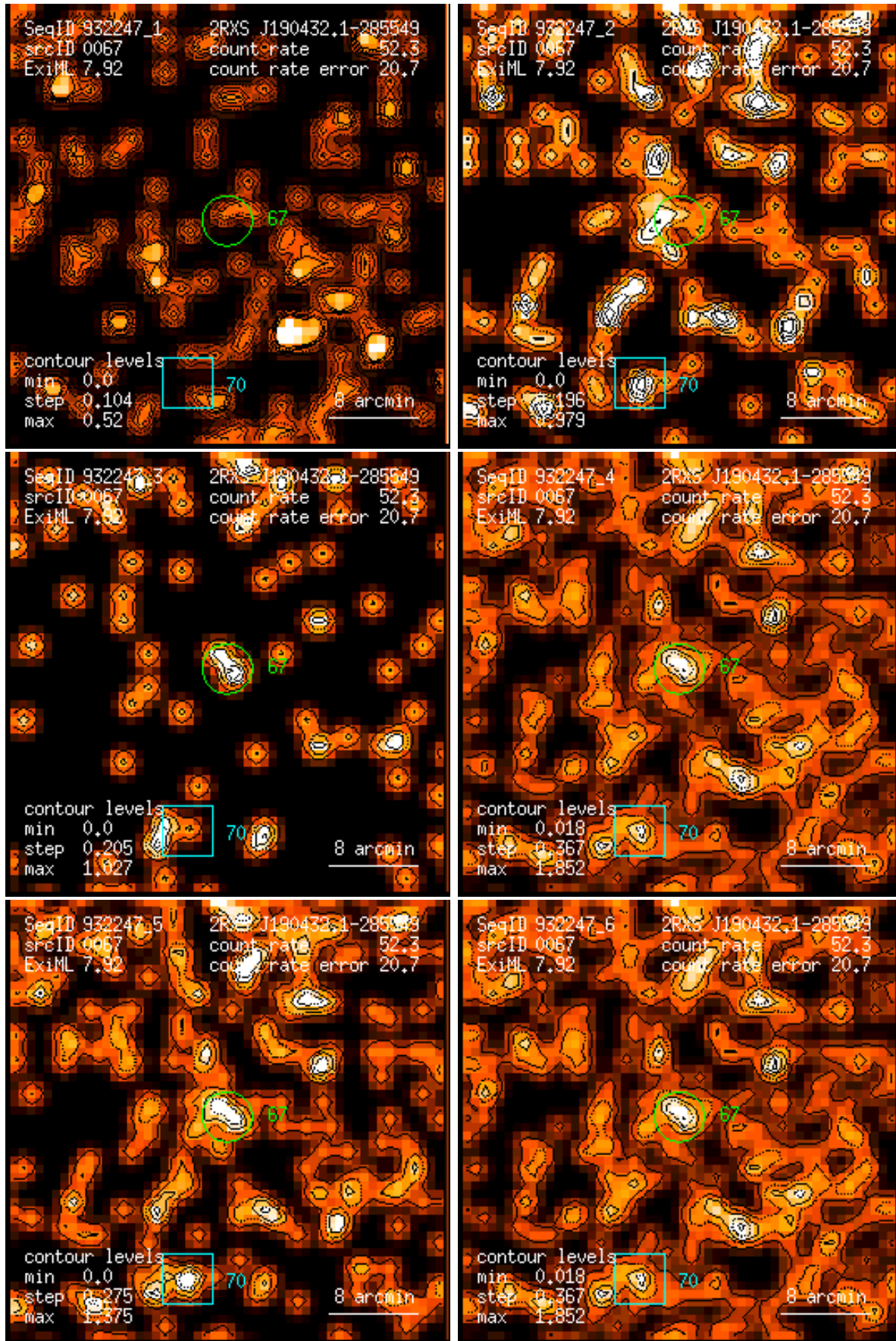
Figure 67: RASS 932247: detection 0067: band rate images, Gaussian filter: (1) PSPC channels 11 – 41, (2) 52 – 90, (3) 91 – 201, (4) 11 – 235, (5) 52 – 201, (6) 11 – 201. Broad band rates in counts/ks. Band rate contour levels in counts/ks/arcmin 2 .
