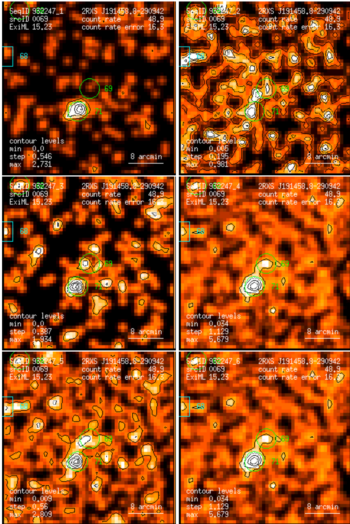
Figure 69: RASS 932247: detection 0069: band rate images, Gaussian filter: (1) PSPC channels 11 – 41, (2) 52 – 90, (3) 91 – 201, (4) 11 – 235, (5) 52 – 201, (6) 11 – 201. Broad band rates in counts/ks. Band rate contour levels in counts/ks/arcmin 2 .
