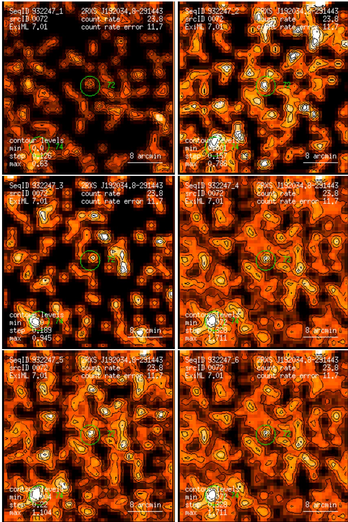
Figure 72: RASS 932247: detection 0072: band rate images, Gaussian filter: (1) PSPC channels 11 – 41, (2) 52 – 90, (3) 91 – 201, (4) 11 – 235, (5) 52 – 201, (6) 11 – 201. Broad band rates in counts/ks. Band rate contour levels in counts/ks/arcmin 2 .
